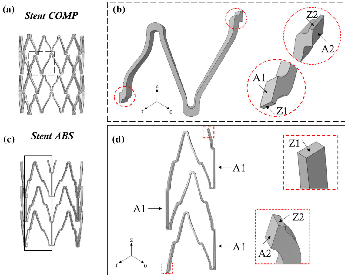
FIGURE 2. (a) The stent COMP geometry with detail of (b) the functional unit; (c) the stent ABS and (d) its functional unit. For both stents, insight into the constrained surfaces of the functional units is given.
