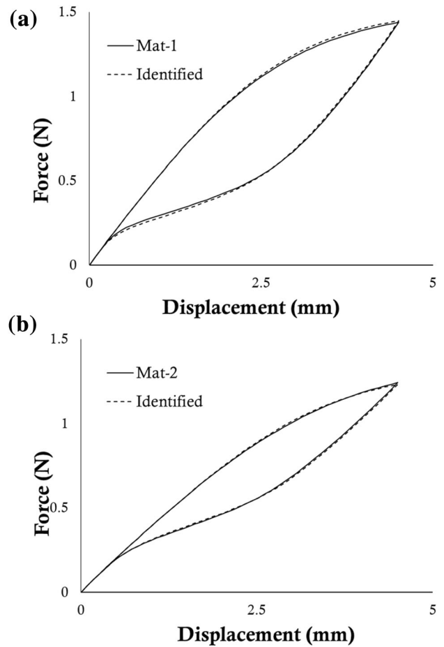
FIGURE 6. Comparison between the tensile force-displacement curves obtained using the target and identified parameters in case of (a) Mat-1 and (b) Mat-2.
