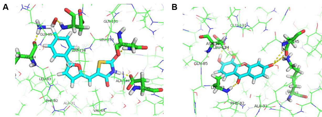
Figure 2 Hydrogen bond positions among amino acid residues of the CDK2 receptor (PDB ID: 2UZ0) with native ligand (A) and with compound 5 (B).
