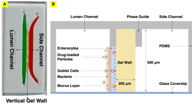
Fig. 1 Mesofluidic gut model enabling visualization of the mucosal interface. (A) Top view, showing 3 channels including a lumen channel in green representing the intestinal lumen, a side channel in red representing circulatory flow, and a gel wall separating them. (B) Schematic cross-sectional view. The apical surface of primary human intestinal epithelial cells cultured on the gel wall faces the lumen. Luminal stimuli (bacteria, particulates, etc.) can be introduced into the lumen channel for studying their interactions with the mucosal barrier.
