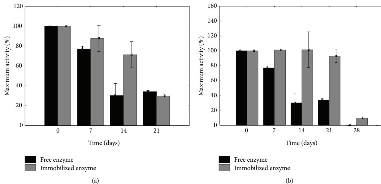
FIGURE 1: Storage stabilities of protocathechuate 3,4-dioxygenase from Stenotrophomonas maltophilia KB2 immobilized in calcium alginate (a) or on glyoxyl agarose (b). Data shown represent the average of three independent trials.
