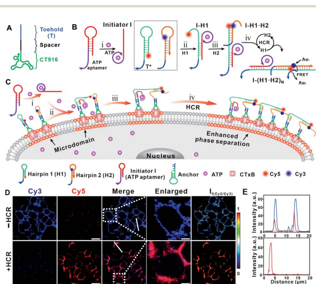
Fig. 1 (A) Structure of the DNA anchor. (B) Scheme of the ATP-activated hybridization chain reaction. (C) Schematic illustration of the ATP-activated hybridization chain reaction on the cell membrane that enhances membrane phase separation. (D) Confocal fluorescence microscopy images of the cells before (top) and after (bottom) HCR treatment. “–HCR” indicates the cells after treatments with CTxB and the DNA anchor and “+HCR” indicates the cells after sequential treatments with CTxB, the DNA anchor and the ATP-activated HCR. The evenly distributed Cy3 fluorescence on the cell membrane was clustered into microdomains upon HCR treatment. The FRET ratio image was obtained from the fluorescence intensity collected in the Cy5/Cy3 channel. Scale bars = 10 μm. (E) Colocalization of Cy3 and Cy5 was analyzed by line profiling the fluorescence intensity along the line selected in confocal images in (D).
