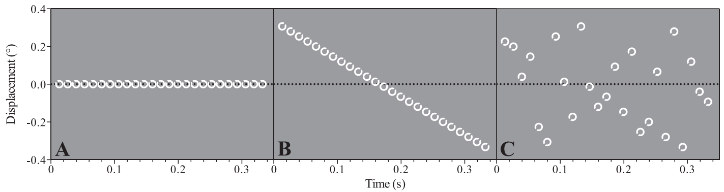
Figure 3. Space-time plots of the motion conditions. Displacement refers to the distance of the target on each frame from a point on the horizontal meridian, 10^\circ to the right of the fixation cross. (A) The target is static. (B) The target is moving sequentially at 2^\circ/s , so is following a smooth path. (C) The target path has been randomized. It can be seen that the individual target locations are identical but are presented in a random order.
