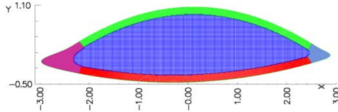
FIG. 5. Computational grid on the eye-shaped domain.
