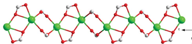
Fig. 2 A one-dimensional chain in 1.
