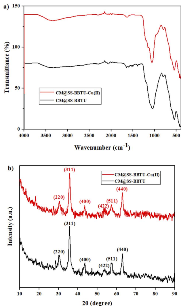
Fig. 1 (a) FT-IR spectra and (b) XRD patterns of CM@SS-BBTU and CM@SS-BBTU-Cu(II).
