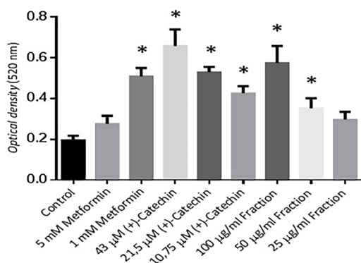
Figure 2. Effect of different concentration of (+)-catechin & proanthocyanidin fraction on the differentiation of 3T3-L1 adipocytes. Data is represented as mean \pm SD, with n = 3 per group. * P \leq 0.05 compared to control.
