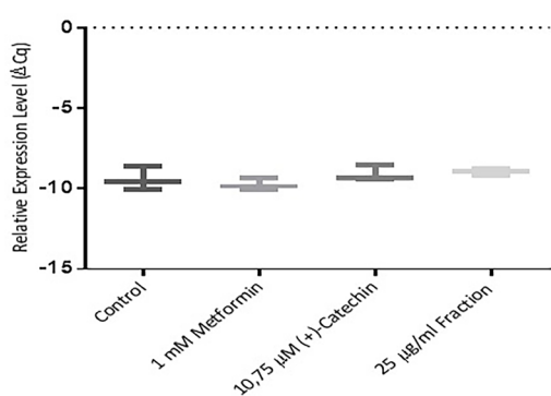
Figure 5. Effect of metformin 1 mM, (+)-catechin (10.75 \mu\text{M} ), proanthocyanidin fraction (25 \mu\text{g}/\text{mL} ) on PPAR \gamma expression. Data is represented as mean \pm SD, with n = 3 per group. *P \leq 0.05 compared to control. Cq : Quantification level.
