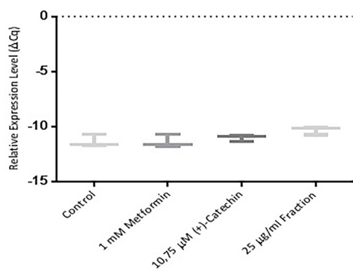
Figure 4. Effect of metformin 1 mM, (+)-catechin (10.75 \mu\text{M} ), proanthocyanidin fraction (25 \mu\text{g}/\text{mL} ) on sirtuin-1 expression. Data is represented as mean \pm SD, with n = 3 per group. *P \leq 0.05 compared to control. Cq : Quantification level.
