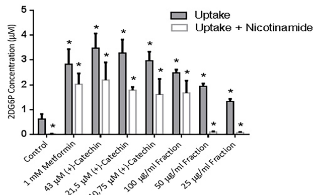
Figure 3. The effects of different concentration of (+)-catechin & proanthocyanidin fraction in glucose uptake of 3T3-L1 adipocytes. Data is represented as mean \pm SD, with n = 3 per group. * P \leq 0.05 compared to control.
