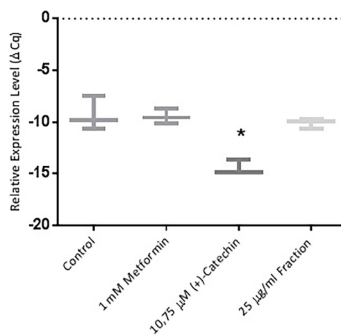
Figure 6. Effect of metformin 1 mM, (+)-catechin (10.75 \mu\text{M} ), proanthocyanidin fraction (25 \mu\text{g}/\text{mL} ) on GLUT-4 expression. Data is represented as mean \pm SD, with n = 3 per group. *P \leq 0.05 compared to control. Cq : Quantification level.
