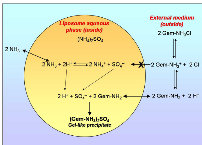
Figure 2 Schematic representation of the gemcitabine encapsulation process within liposomes by means of the presence of a pH gradient elicited by the co-encapsulation of a 250 mM ammonium sulphate solution.
