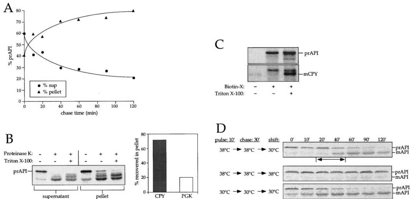
Figure 5. The membrane accumulation phenotype of the K12R API ts mutant is thermally reversible. (A) K12R API accumulates in the pellet fraction at nonpermissive temperature. Spheroplasts were labeled for 10 min at 38°C followed by nonradioactive chase. Aliquots were removed at the indicated chase times and separated into supernatant ( sup ) and pellet fractions. Samples were immunoprecipitated with antiserum to API, and the radiolabeled signals were quantitated. The percent radiolabeled precursor at a given chase point represents the ratio of precursor from each supernatant or pellet fraction to the total API combined in both fractions. (B) Protease accessibility of K12R API in the supernatant and pellet fractions. Spheroplasts were labeled for 5 min, chased for 30 min at 38°C, and separated into a supernatant and pellet fraction after differential osmotic lysis. The supernatant and pellet fractions were subjected to proteinase K and Triton X-100 as indicated and immunoprecipitated with antiserum to API ( left ). An aliquot of the recovered pellet fraction was also immunoprecipitated with antisera to the vacuolar marker CPY and the cytosolic marker PGK before protease treatment ( right ). The percent of marker proteins recovered in the pellet fraction was calculated as described for Fig. 3. (C) Accessibility of K12R API in the pellet fraction to cross-linking with Sulfo-NHS-biotin. Labeled spheroplasts were fractionated exactly as in B. The pellet fraction was cross-linked with Sulfo-NHS-biotin ( Biotin-X ) in the presence or absence of Triton X-100. API and CPY were recovered by immunoprecipitation followed by precipitation with avidin agarose beads. (D) Thermal reversibility of the K12R API membrane-accumulation phenotype. The K12R API mutant was pulse-labeled for 10 min, chased for 30 min at 38°C, and then shifted to 30°C ( top ). Samples were removed at the indicated times during the shift period at 30°C and lysed with glass beads. The resulting cell extracts were immunoprecipitated with antiserum to API and resolved by SDS-PAGE. The double-headed arrow in the top panel marks the 20–40-min window of time when mature API increases from 10 to 56% during the 30°C shift. The K12R API strain was also pulse labeled, chased, and incubated all at 38°C ( middle ) or 30°C ( bottom ) in this experiment.
