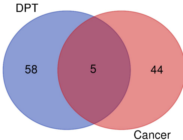
Fig. 5 Venn diagram between the overexpressed genes and the three genes associated with aspirin
