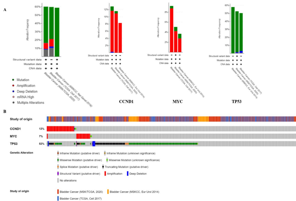
Fig. 2 Analysis of genetic alterations of 3 DPTs of aspirin (CCND1, MYC and TP53) in human bladder cancer studies embedded in cBio cancer genomics portal. A Overview of the changes in CCND1, MYC and TP53 in genomics datasets available in 3 different studies. B Visual summary of mutations across a set of human bladder cancer samples based on a query of the 3 genes in OncoPrint. Distinct genomic alterations including mutations, copy number alterations, exemplified by gene amplifications and homozygous deletions, are summarized and color coded (as % changes) in the affected genes in individual tumor samples. Each row represents a gene, and each column represents a tumor sample
