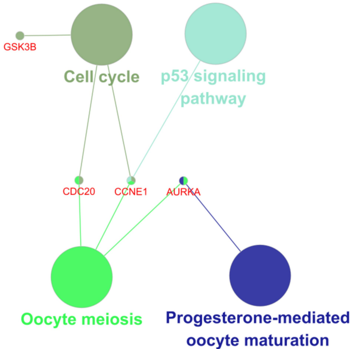
Fig. 6 KEGG pathway analysis of aspirin related four predictive targets of bladder cancer
