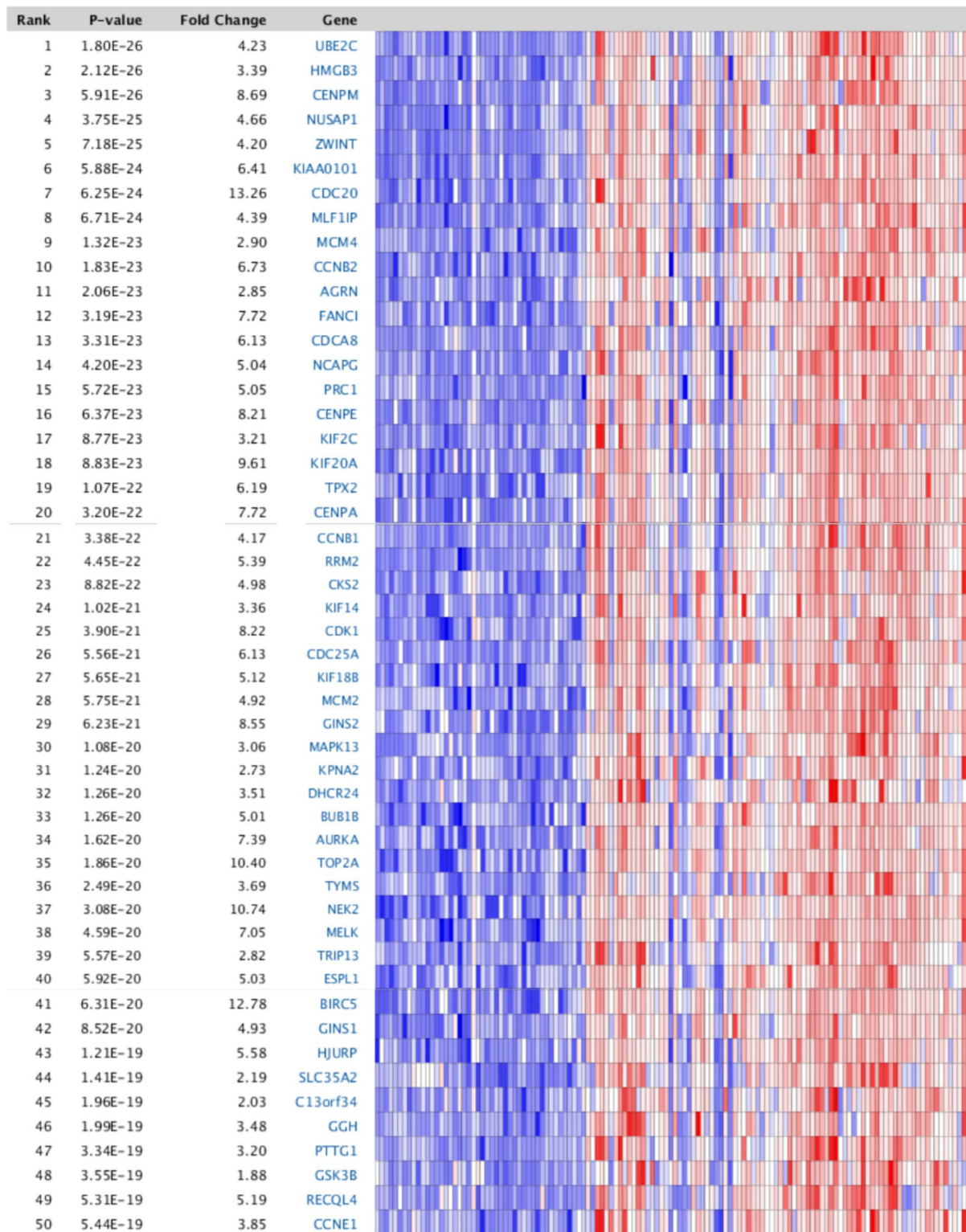
Fig. 4 The top 50 over-expressed genes in bladder cancer vs. normal tissue using the Oncomine database
