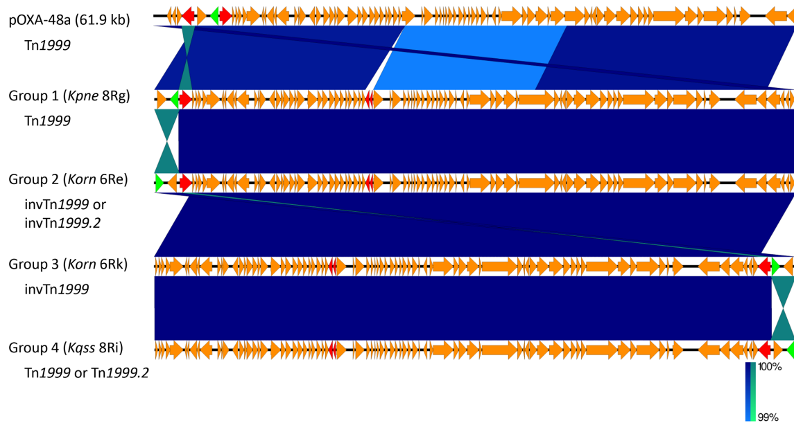
Fig. 4. Alignment of pOXA-48 ([17]; accession no. JN626286) and representative contigs from our isolates harbouring bla OXA-48 . Arrows represent ORFs; bla OXA-48 is shown in green and insertion sequences in red.
