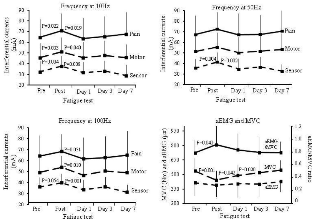
Fig. 2. Changes of the thresholds of interferential currents at different frequencies and aEMG/MVC after fatigue test and during recovery in male sprinters. Abbreviations: MVC = maximal voluntary contraction; aEMG = amplitude of surface electromyography.
