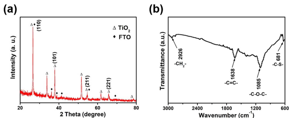
Fig. 1 (a) XRD pattern and (b) FTIR spectra of \text{TiO}_2/\text{PEDOT} film.
