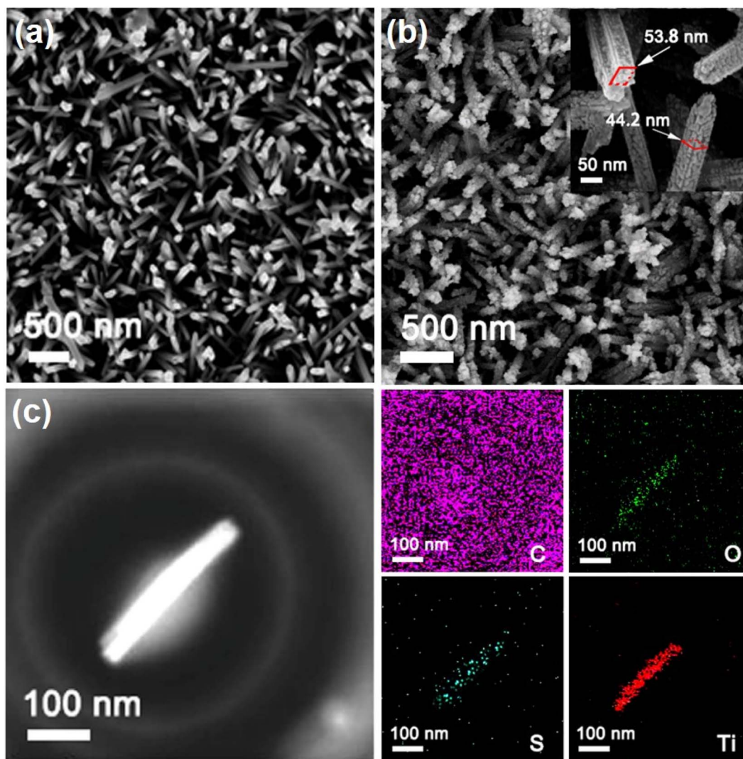
Fig. 2 Top-view scanning electron microscope (SEM) images of (a) \text{TiO}_2 and (b) \text{TiO}_2/\text{PEDOT} nanorod arrays. (Inset) The \text{TiO}_2/\text{PEDOT} nanorod arrays details of partial enlarged. (c) TEM images and EDS elemental maps of the \text{TiO}_2/\text{PEDOT} nanorod.
