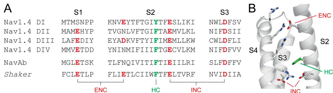
Figure 1. Highly conserved acidic and aromatic side chains in the VSDs of voltage-gated ion channels. (A) Sequence alignment of S1, S2, and S3 segments of different voltage-gated ion channels: Na_v 1.4, NavAb, and Shaker potassium channels. The S2 HC is highlighted in green; negatively charged side chains in the ENC and the INC are highlighted in red. (B) Structure of the Na_v Ab VSD (Protein Data Bank accession no. 3RVY; Payandeh et al., 2011). The conserved S4 arginines, as well as conserved acidic and aromatic side chains in S2 and S3, are shown in stick representation (note that S1 was omitted for clarity).
