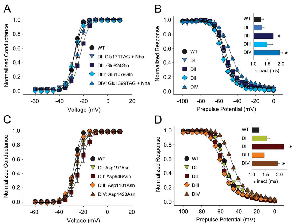
Figure 3. Removing the negative charge in the INC has little effect on channel activation. (A and B) G-V (A) and SSI curves (B) for WT and mutants in which the S3 INC was neutralized through introduction of Nha or Gln (DI, Glu171TAG + Nha; DII, Glu624Gln; DIII, Glu1079Gln; DIV, Glu1399TAG + Nha). (C and D) G-V (C) and SSI curves (D) for WT and mutants in which the S3 INC was neutralized through the introduction of Asn (DI, Asp197Asn; DII, Asp646Asn; DIII, Asp1101Asn; DIV, Asp1420Asn). The insets in B and D show bar graphs representing the average time constants for fast inactivation ( \tau ) for a depolarizing voltage step to -15 mV. *, statistical difference to WT values in an unpaired t test ( P < 0.01 ).
