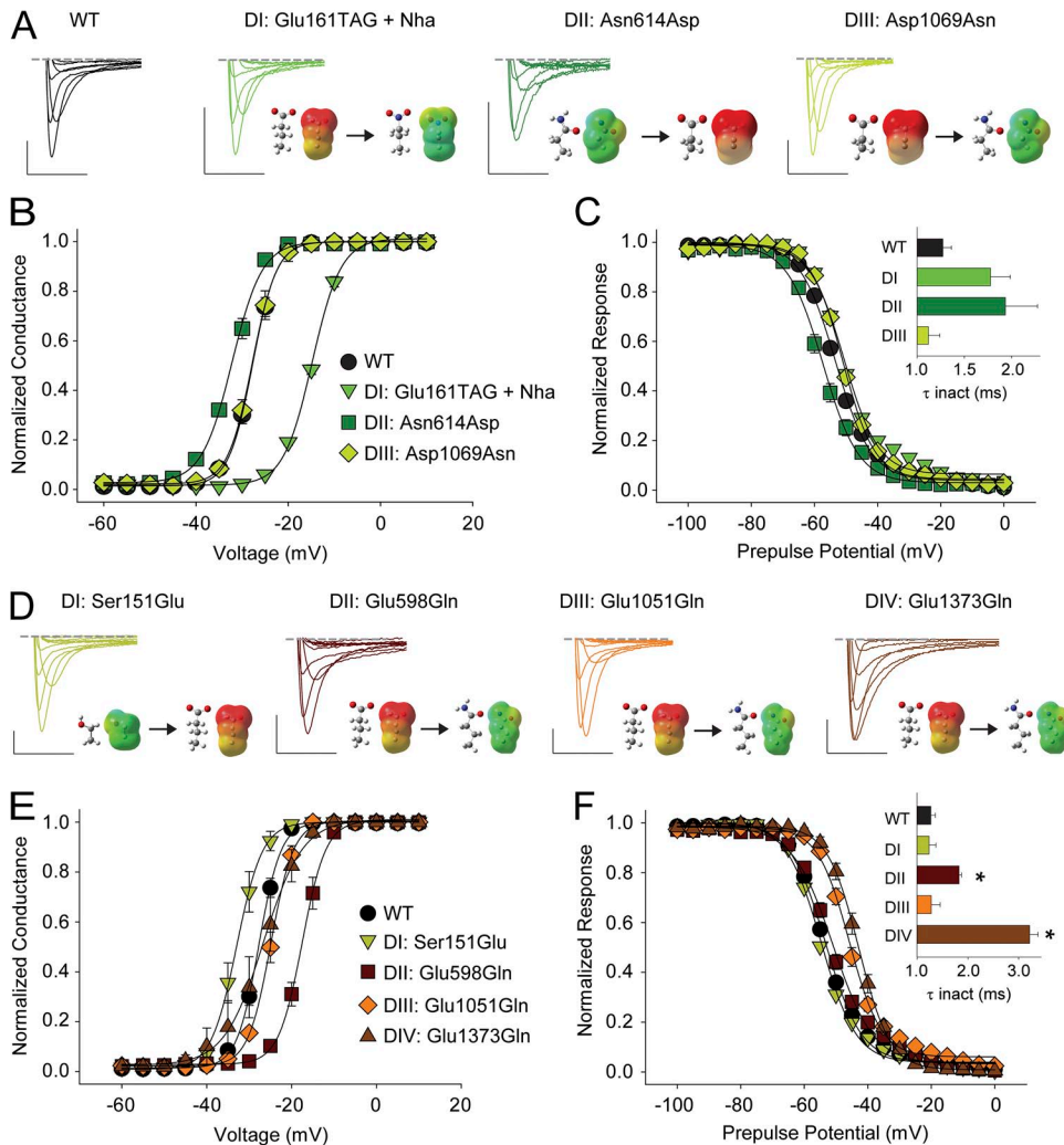
Figure 2. ENC electrostatic contributions are critical in DI and DII only. (A and D) Sample traces for currents recorded for WT and mutants at the S1 and the S2 ENC in DI–DIV. (B, C, E, and F) G-V (B and E) and SSI curves (C and F) for WT and mutants at the S1 and the S2 ENC; the insets in C and F show a bar graph representing the average time constants for fast inactivation ( \tau ) for a depolarizing voltage step to -15 mV for WT and the mutants; *, statistical difference to WT values in an unpaired t test ( P < 0.01 ). Note that Asn1389 in the S2 ENC in DIV had been mutated to both acidic and basic side chains previously with no functional consequence and was thus not studied further here (Groome and Winston, 2013). Bars: horizontal, 5 ms; vertical, 200 nA. Voltage steps were from -40 to +20 mV in 10-mV increments. Insets show energy-minimized structures and ESP maps of side chains (red, -100 kcal/mol; green, 0 kcal/mol; blue, +100 kcal/mol; see Pless et al., 2011b, for details).
