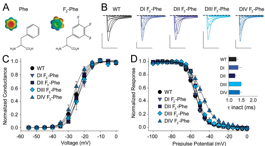
Figure 5. Removing the negative ESP of the S2 aromatic has minimal functional consequences. (A) Chemical structures and ESP maps of Phe and 3,4,5-trifluoro-Phe (F 3 -Phe) (ESP: red, -25 kcal/mol; green, 0 kcal/mol; blue, +25 kcal/mol; see Pless et al., 2011a, for details). (B) Sample traces for currents recorded from WT or mutants in which F 3 -Phe has been introduced in the S2 HC (DI, Tyr168TAG + F 3 -Phe; DII, Phe621TAG + F 3 -Phe; DIII, Phe1076TAG + F 3 -Phe; DIV, Phe1396TAG + F 3 -Phe). Bars: horizontal, 5 ms; vertical, 500 nA. Voltage steps were from -40 to +20 mV in 10-mV increments. (C and D) G-V (C) and SSI curves (D) for WT and mutants in which the S2 aromatic was replaced by F 3 -Phe; the inset in D shows a bar graph representing the average time constants for fast inactivation ( \tau ) for a depolarizing voltage step to -15 mV for WT and the F 3 -Phe mutants in DI–DIV.
