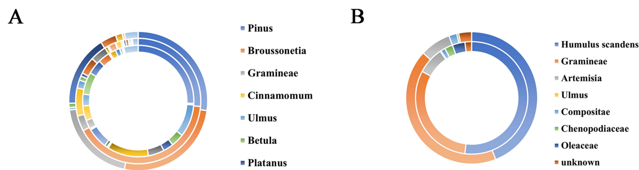
Figure 3 Ring diagram traces airborne presence. (A) A ring structure to visually represent the proportional airborne pollen presence in Suzhou across the months of March, April, and May. The innermost circle provides insights into pollen distribution during March, the middle circle illustrates the distribution for April, and the outermost circle showcases the distribution during May. (B) The relative proportion of airborne pollen presence in Suzhou during the months of September and October. The innermost circle reflects the distribution for September, while the outermost circle highlights the distribution observed in October.
