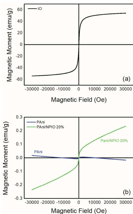
Fig. 8 Magnetization curves of (a) IO and (b) pure PANi and the PANi/NPIO 20% composite.
