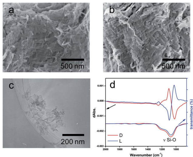
Fig. 1 SEM images of calcined silicas, (a) D - \text{SiO}_2 -600 and (b) L - \text{SiO}_2 -600. TEM images of (c) the piece of L - \text{SiO}_2 crushed by homogenizing the methanol solution containing chiral silica bundles (calcined PEI/tart@ \text{SiO}_2 ) for at least 20 000 rpm for 2 min. (d) FT-IR/VCD spectra of the crushed \text{SiO}_2 , red lines for the D -form, and blue lines for the L -form.
