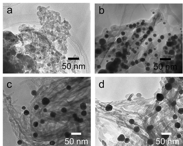
Fig. 2 TEM images of (a) D -, (b) L - \text{Ag@SiO}_2 -500 and (c) D -, (d) L - \text{Au@SiO}_2 -500.
