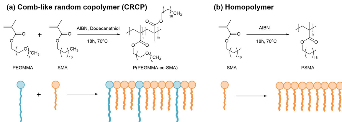
Scheme 2 Syntheses of (a) comb-like random copolymers of P(PEGMMA- co -SMA) and (b) a homopolymer of PSMA.
