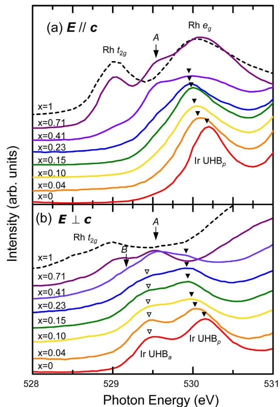
Figure 3. Low energy parts in the O K -edge XAS spectra with (a) E // c and (b) E \perp c , where c is the surface normal axis. The spectra of \text{Sr}_2\text{RhO}_4 were taken from ref. 27. The E \perp c spectra are reproduced from the \sigma -polarisation data, and the E // c spectra are deduced from the relation: I_{E // c} = \frac{I_{\pi} - \cos^2 60^\circ I_{\sigma}}{\sin^2 60^\circ} . Solid (open) triangles highlight the peak positions of the \text{Ir } J_{\text{eff}} = 1/2 UHB hybridised with the in-plane (apical) O 2p .
