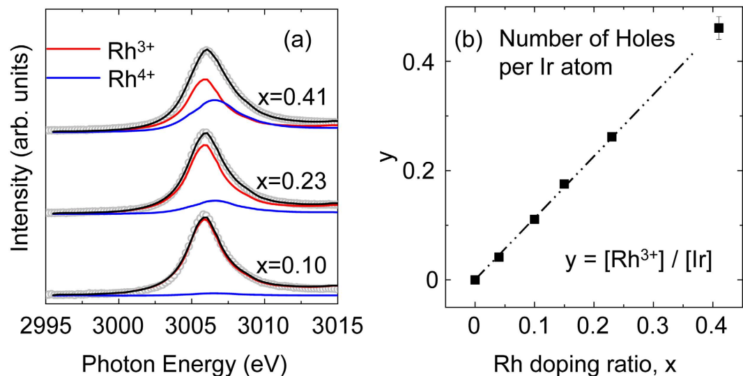
Figure 1. (a) Rh L_3 -edge XAS spectra of \text{Sr}_2\text{Ir}_{1-x}\text{Rh}_x\text{O}_4 crystals of x = 0.10, 0.23 and 0.41 . The open circles show the experimental spectra and the black solid curves show the fitting results. The spectra of \text{Rh}^{3+} in \text{Rh}_2\text{O}_3 (red curve) and \text{Rh}^{4+} in \text{Sr}_2\text{RhO}_4 (blue curve) were taken from ref. 26 for the fitting. (b) The deduced values of \text{Rh}^{3+} concentration per one Ir site as a function of Rh doping ratio ( x ). Almost linear relation manifests the hole doping scheme at least for x \leq 0.23 . The error bars account for the uncertainty in determining the peak areas.
