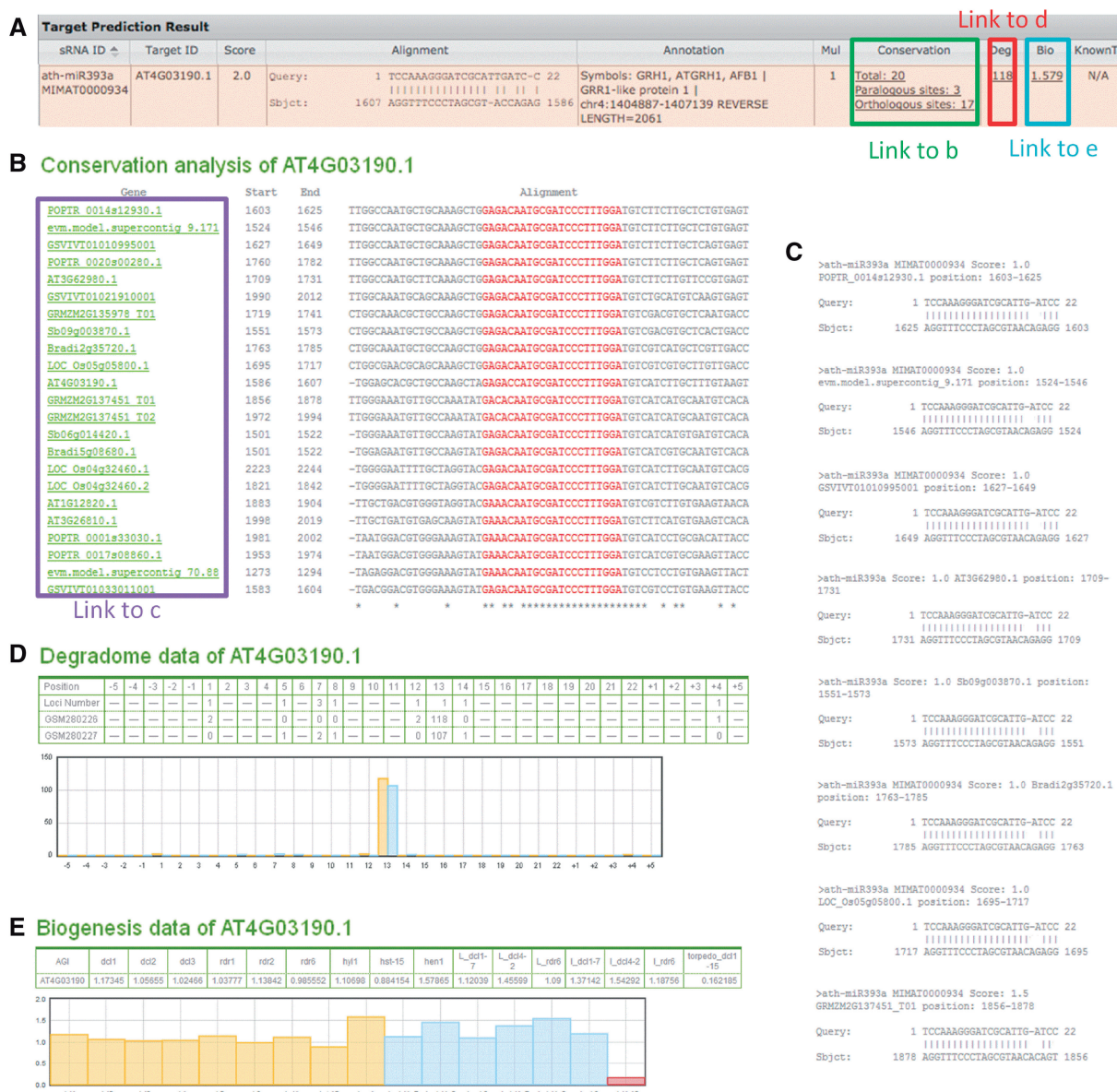
Figure 3. Illustration of expandable links in the target prediction result table. (A) A sample line of the target prediction result table; (B) target site conservation analysis results. Homolog genes with the same smRNA target site, both within and cross-species, are shown in the ClustalW multiple alignment format; (C) the alignments between miRNA and targets provoked by mousing over the hyperlinks of gene IDs listed in (B); (D) Degradome data of the predicted smRNA target. Positions listed in the table are orders of nucleotides in the smRNA sequences, plus upstream and downstream 5 nt each; ‘Loci number’ represents the number of perfectly mapped loci of each degradome sequence, marked at the start nucleotide position of each sequence. Normalized reads starting at each nucleotide position in the degradome data are listed in following rows. The histogram shows the distribution of the degradome reads. In the example, the target should be cleaved after the 12th nucleotide according to the degradome data; (E) Expression change of target gene in smRNA biogenesis pathway gene mutants compared to wild-type plants. Fold changes of the normalized expression values between mutants and wildtype are shown in the table and the Y axis of the plot. Data from different datasets are distinguished by colors in the plot.
