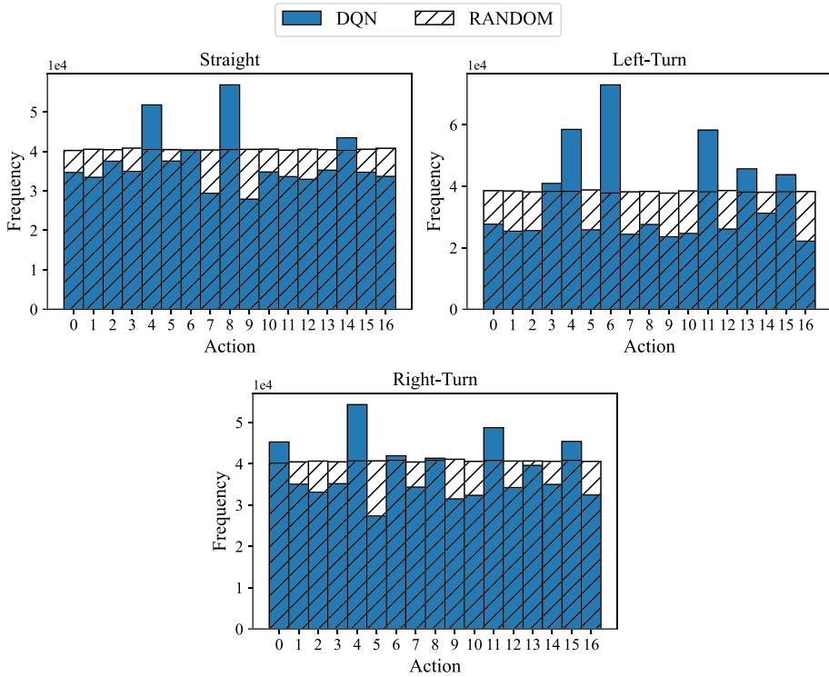
Fig. 13 Actions distributions (DCL requirement)
