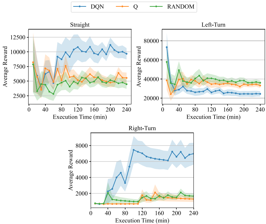
Fig. 7 Average reward over time (DV requirement)
