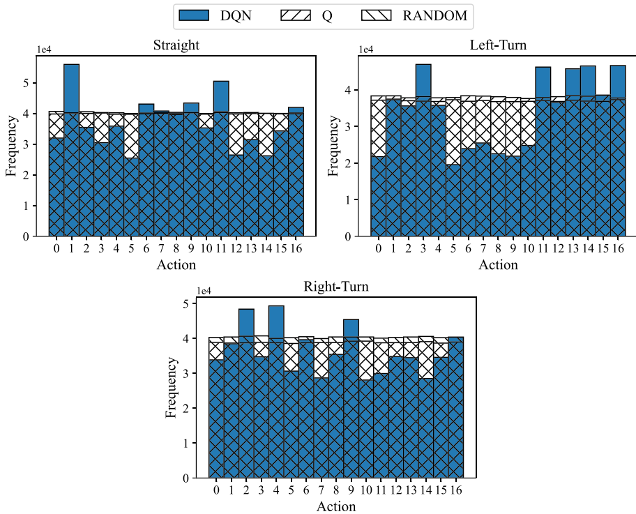
Fig. 8 Action distributions (DV requirement)
