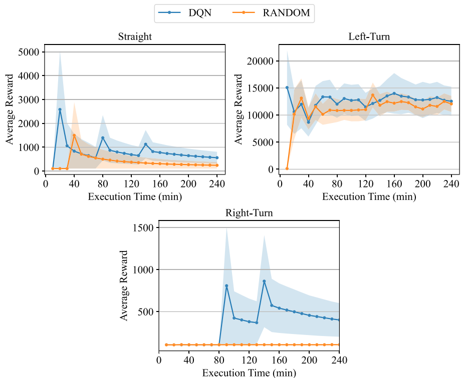
Fig. 12 Average reward over time (DCL requirement)
