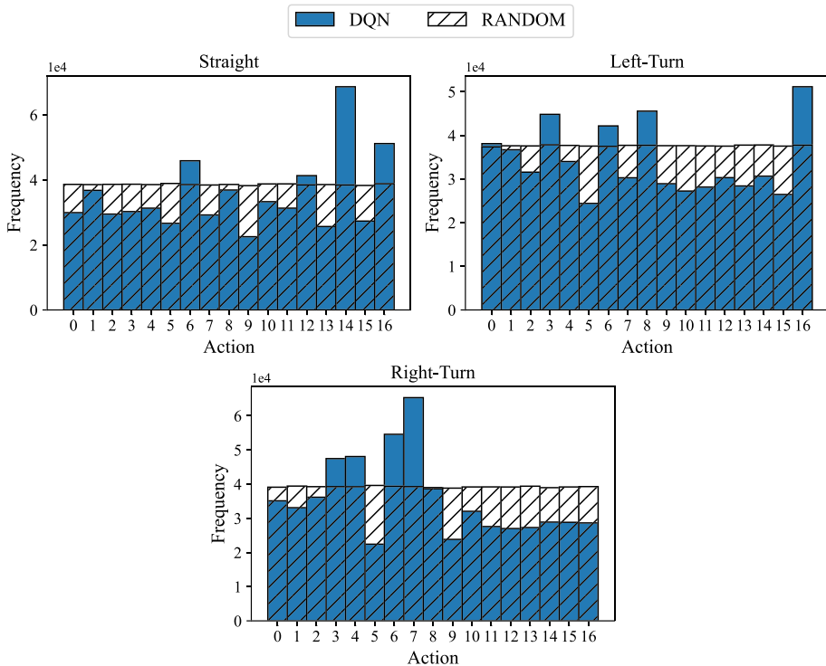
Fig. 17 Actions distributions (DP requirement)
