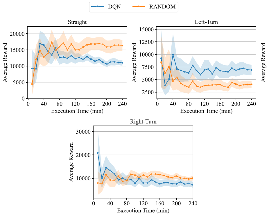
Fig. 16 Average reward over time (DP requirement)
