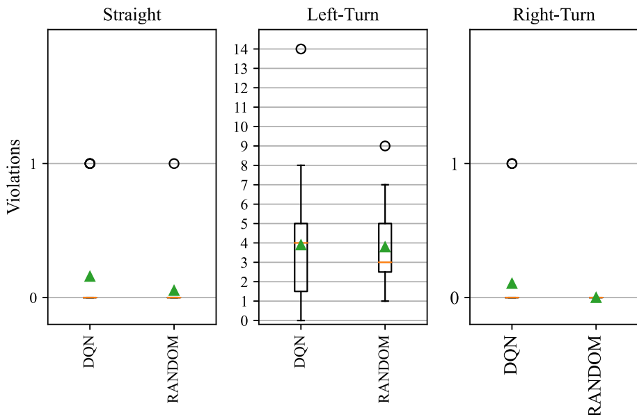
Fig. 10 Box plots of the number of violations of the DCL requirement
