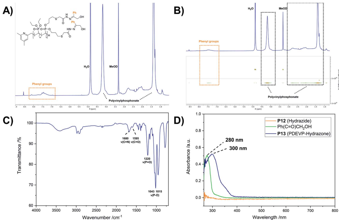
Fig. 7 ^1\text{H-NMR} spectrum of P13 in MeOD (A) and corresponding DOSY (B) as well as IR spectrum of P13 (C). UV/Vis spectra of the hydrazide P12 (100 \mu\text{M} with respect to the ally groups), 2-hydroxyacetophenone ( 7 ) (500 \mu\text{M} ) and the hydrazone conjugate P13 (100 \mu\text{M} with respect to the phenyl groups) in methanol (D).
