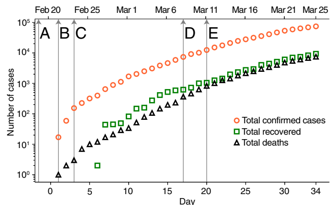
Fig. 2. Time evolution of the COVID-19 epidemic in Italy. Time marks are as follows: a, the first patient with suspected local transmission is hospitalized in Codogno; b, first confirmed cases; and c, d, and e, main containment measures enforced by the Italian government (detailed in Materials and Methods ).
