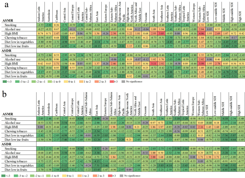
Figure S3. The AAPC for EC risk attributable ASMR and ASDR for males
