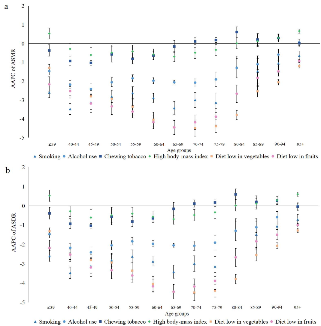
Figure S2. The AAPCs of ASMR (a) and ASDR (b) for females in age groups in 1990-2019, globally. (AAPC: average annual percentage change; ASMR: age-standardized mortality rate; ASDR: age-standardized DALY rate.)
