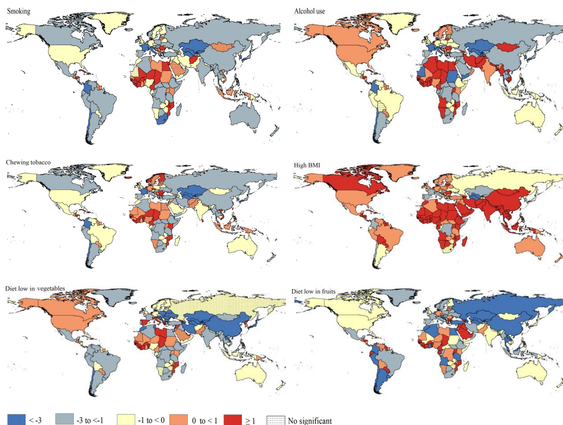
Figure S6. The AAPC of EC ASDR attributable to specific risk factors for males at 204 countries and territories from 1990 to 2019.
