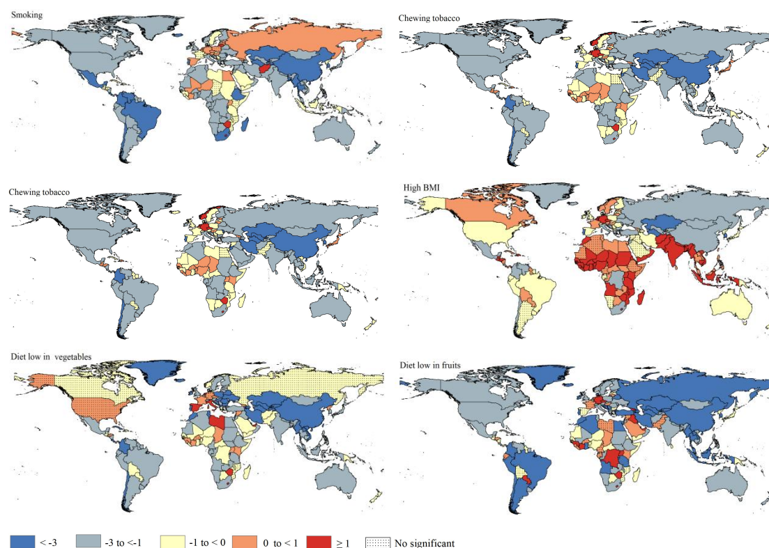
Figure S7. The AAPC of EC ASDR attributable to specific risk factors for females at 204 countries and territories from 1990 to 2019
