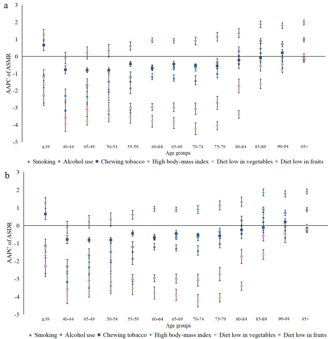
Figure S1. The AAPCs of ASMR (a) and ASDR (b) for males in age groups in 1990-2019, globally. (AAPC: average annual percentage change; ASMR: age-standardized mortality rate; ASDR: age-standardized DALY rate.)
