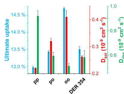
Figure 6. Chemical performance in methanol of networks produced using MXDA as the amine monomer and para-para - (pp), para-ortho - (po), and ortho-ortho - (oo)-DGEBF or Dow Epoxy Resin 354 (DER 354) as the epoxide monomer. Shown are the ultimate uptake (by original mass) of each network and the diffusion coefficients of sorption ( D_{sor} ) and desorption ( D_{des} ) at 40 °C. Error bars show standard error of the three samples.
