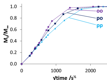
Figure 7. Methanol sorption profiles of DGEFB/MXDA networks made with the different isomers of DGEFB [para-para- (pp), para-ortho- (po), and ortho-ortho (oo)]. The individual data points are shown joined with straight lines.
