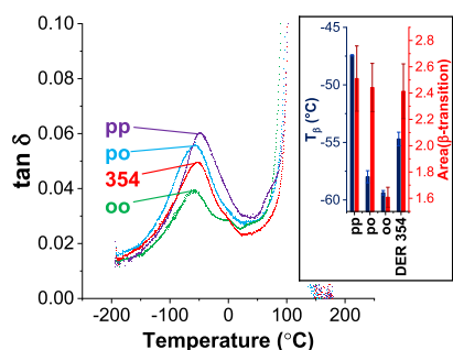
Figure 5. DMA measurement of \tan \delta vs temperature, showing the \beta -transition for the networks produced using MXDA as the amine monomer and para-para - (pp), para-ortho - (po), and ortho-ortho - (oo)-DGEBF or Dow Epoxy Resin 354 (DER 354) as the epoxide monomer. Inset: the T_\beta and area of the peak associated with the \beta -transition for each of the networks. Error bars show standard error of two samples.
