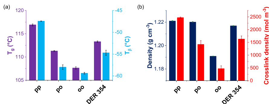
Figure 4. Physical properties of networks produced using MXDA as the amine monomer and para-para - (pp), para-ortho - (po), and ortho-ortho - (oo)-DGEBF or Dow Epoxy Resin 354 (DER 354) as the epoxide monomer. (a) Glass transition temperature ( T_g ), the \beta -transition temperature ( T_\beta ) as determined by DMA and (b) crosslink density as determined by DMA (calculated from eq 2—see Experimental Section) and density as determined by helium pycnometry. Error bars show standard error for three samples for T_g and crosslink density, standard error for two samples for T_\beta , and standard deviation of ten measurements of a single sample for density.
