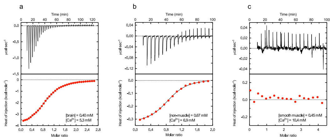
Figure 3 Representative isothermal calorimetry thermograms for calcium binding to \alpha -actinin 1 C-terminal domains. Heat traces were obtained by injecting calcium chloride to brain (A), non-muscle (B) or smooth muscle (C) isoform, using the indicated concentrations of protein and calcium. After integration, a single-site-binding isotherm was fitted to the data to obtain the enthalpy of binding \Delta H , entropy \Delta S and the dissociation constant K_d . Best fitting dissociation constants for the calcium binding to the brain or non-muscle isoforms were 44.8 and 54.7 \mu\text{M} , respectively, for the data displayed in the figure. The first point in ITC titration was not included in the fitting. Data shown are representative of at least 10 independent experiments. In all figures, red circles represent experimental data and the full drawn line the best fit.
