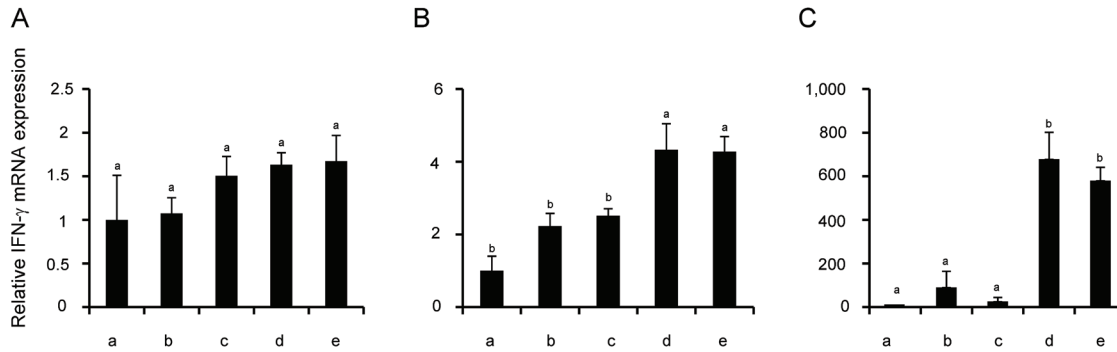
Fig. 3. IFN-γ mRNA expression in (A) spleen, (B) iliac lymph node, and (C) vaginal tissue after vaginal herpes simplex virus (HSV) infection in mice administered with Korean red ginseng (KRG) extract. KRG administered mice ( n=7 ) were intravaginally challenged, and each organ was collected on day 2 after virus infection. IFN-γ mRNA was measured by real time polymerase chain reaction and relative expression levels were normalized. (a) Mock control, (b) HSV infected control, (c) KRG 100 mg/kg, (d) KRG 200 mg/kg, and (e) KRG 400 mg/kg. Data are presented as means±SEM for each group. Different letters indicate significant differences ( p<0.05 ) according to Duncan's multiple range test.
