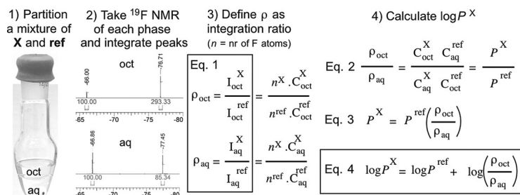
Figure 1. Principle of the \log P determination method. See the Supporting Information for a detailed procedure.
