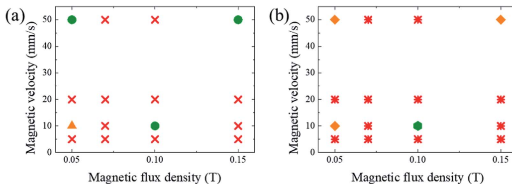
Fig. 6 Phase diagrams for optimal conditions with lowest deviation. (a) Phase diagram for the average spatial deviation on y -axis with respect to helical diameter, D_h . Green circles (●): \overline{D}_y < D_h . Orange triangles (▲): D_h < \overline{D}_y < 2D_h . Red × (×): \overline{D}_y > 2D_h . (b) Phase diagram for average temporal deviation with respect to time for displacement of the helix diameter, t_D . Green hexagons (⬡): \overline{\Delta t} < t_D . Orange diamonds (◆): t_D < \overline{\Delta t} < 2t_D . Red asterisks (*): \overline{\Delta t} > 2t_D .
