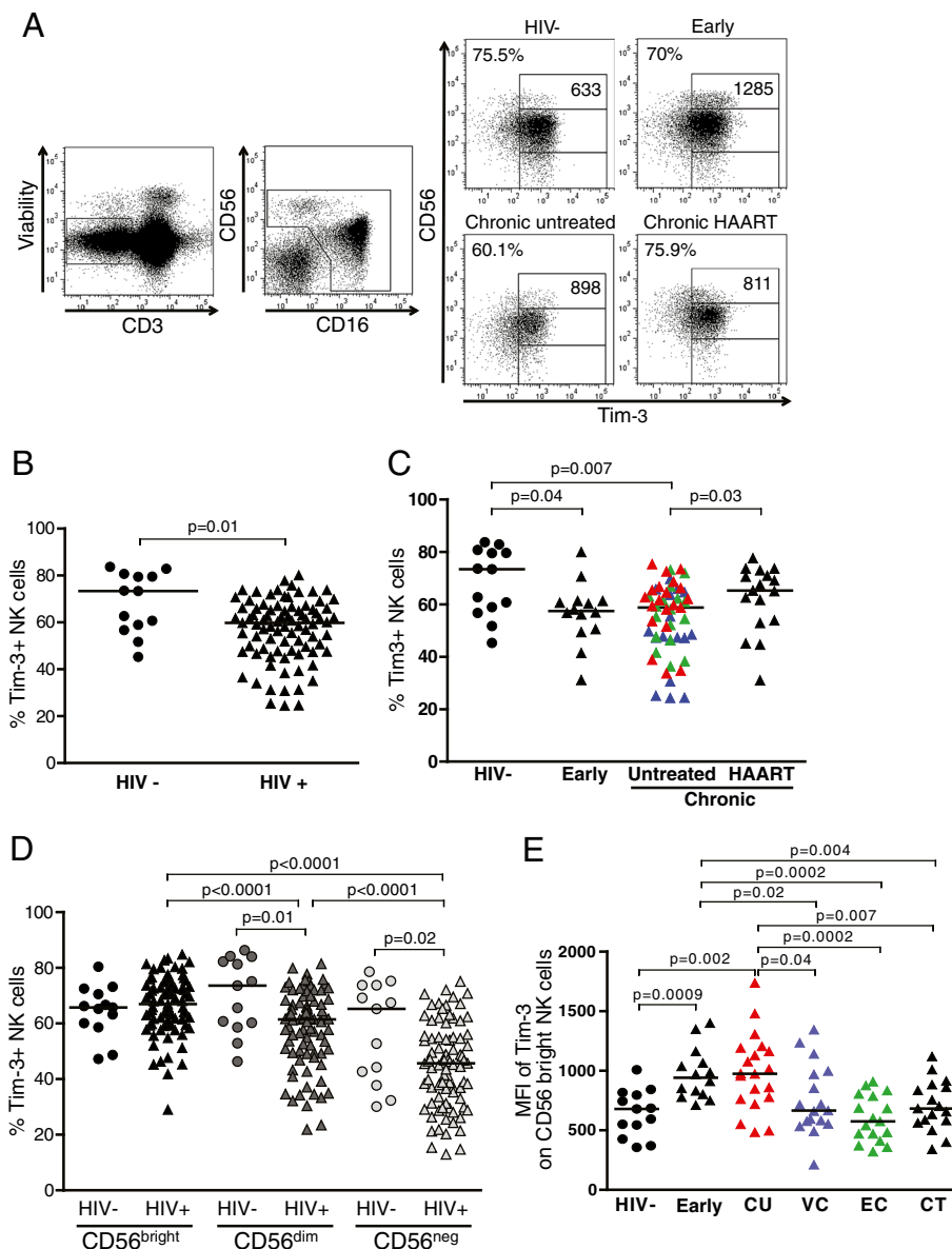
Figure 1 Tim-3 expression is dysregulated in HIV-1 infection. (A) Flow cytometry gating strategy: Gates are set to include CD3 + lymphocytes and exclude dead cells (viability marker + ). NK cell subsets are defined by the expression of CD56 and CD16, and Tim-3 + NK cells by using appropriate fluorescence-minus-one controls. The four right flow cytometry panels show representative examples of Tim-3 + bulk and CD56 bright , CD56 dim and CD56 neg NK cells in an HIV-1 negative subject (HIV-), an individual with late primary untreated infection, an untreated chronic HIV-1 progressor, and a HAART-treated HIV-1+ patient. Percentages of Tim-3 + bulk NK cells, and MFI of Tim-3 on CD56 bright NK cells are indicated on the top left of the main panel and on the top right of the CD56 bright NK cell gate, respectively. (B) Dot plots represent the percentage of Tim-3 + NK cells from 13 healthy individuals and 85 HIV-1-infected subjects (C) , including 14 with early untreated HIV-1 infection, 54 with chronic untreated HIV-1 infection (blue, 17 viremic controllers; green, 17 elite controllers; red, 20 untreated progressors), and 17 with HAART-treated HIV-1 infection. (D) Percentages of Tim-3 + NK cells in CD56 bright (CD3 + CD56 + CD16 - ), CD56 dim (CD3 + CD56 + CD16 + ) and CD56 neg (CD3 + CD56 - CD16 + ) NK cells in 13 HIV-1 negative and 85 HIV-1-infected subjects. (E) MFI of Tim-3 on CD56 bright NK cells in 13 healthy individuals and 14 subjects with early infection, 54 with chronic untreated HIV-1 infection, including 17 viremic controllers (blue, VC), 17 elite controllers (green, EC), 20 untreated progressors (red, CU), and 17 with HAART-treated HIV-1 infection (CT). Horizontal lines indicate the median percentages. Statistical differences with p < 0.05 are indicated and were determined using the Mann-Whitney t test to compare phenotype frequencies between two groups.
