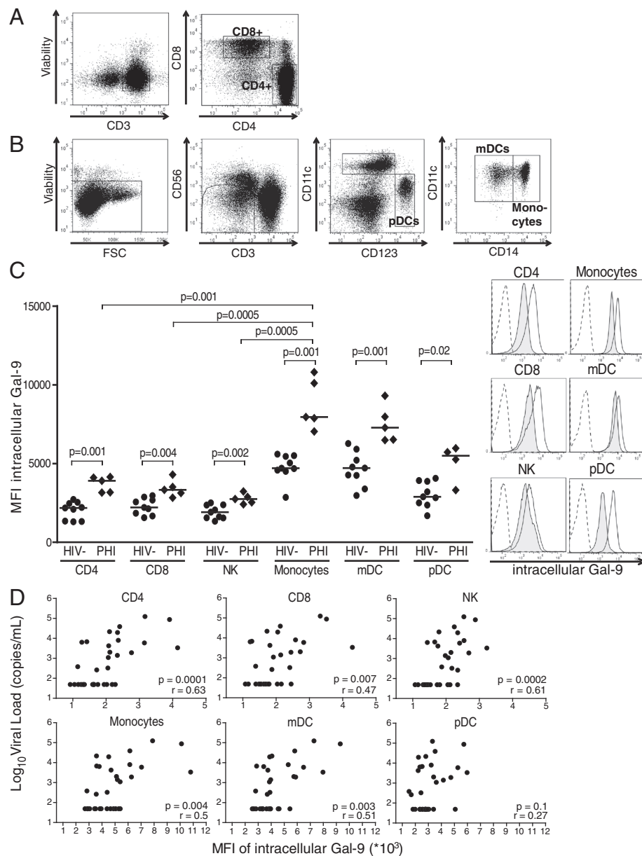
Figure 3 Expression of galectin-9 in PBMCs is increased in early HIV-1 infection and correlates with HIV-1 viremia. Flow cytometry gating strategy to analyze intracellular expression of Gal-9 on (A) CD4+ and CD8+ T cells and (B) pDCs, monocytes or mDCs. Gates are set to exclude dead cells (viability marker + ), and expression of Gal-9 on various lymphocyte subsets is defined by using appropriate fluorescence-minus-one controls. (C) Dot plots display the MFI of intracellular Gal-9 in the indicated immune cell subsets from 9 healthy (HIV-) and 5 untreated subjects with early infection as determined by flow cytometry. Horizontal lines indicate the median percentages. Differences where p < 0.05 are indicated. Histogram overlays display representative examples of intracellular Gal-9 expression in each lymphocyte subset analyzed in healthy controls (tinted) and in individuals with early HIV-1 infection (transparent) compared to the FMO (dotted line). PHI, early HIV-1 infection (D) Correlations between the logarithmic viral load and the MFI of intracellular Gal-9 in CD4+ T cells, CD8+ T cells, NK cells, monocytes, mDCs and pDCs from a subset of 32 HIV-1-positive individuals, including 4 subjects with early infection, 6 viremic controllers, 6 elite controllers, 9 subjects with chronic untreated, and 7 with chronic treated HIV-1 infection.
