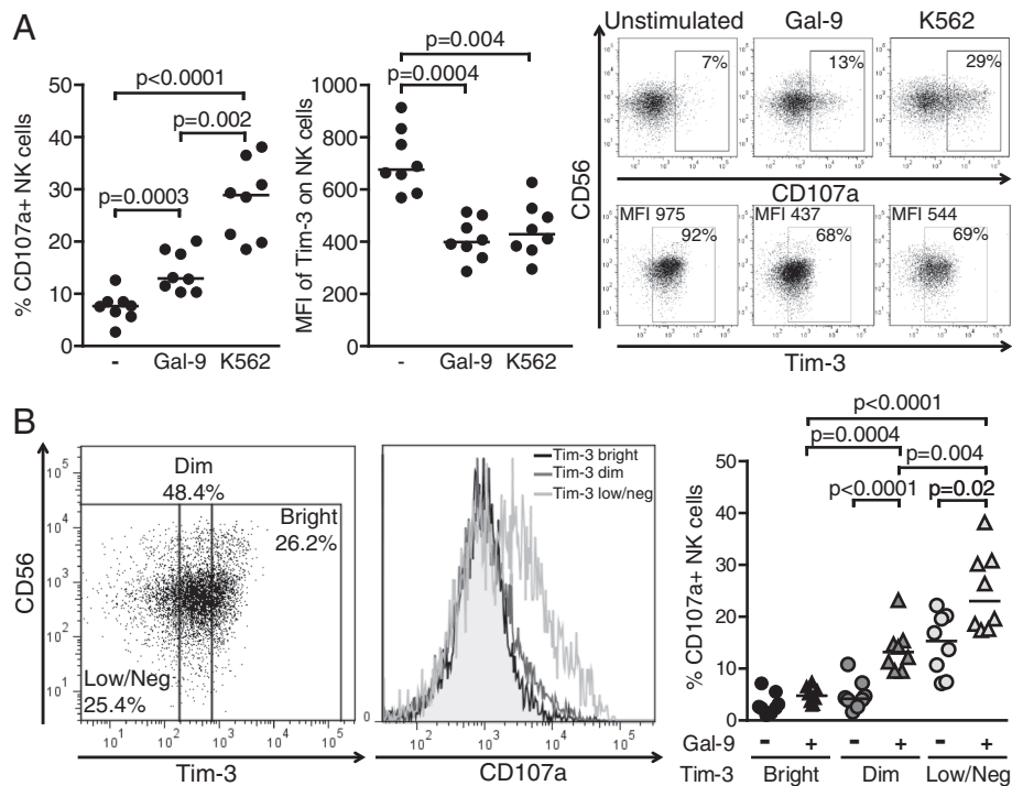
Figure 4 Incubation with soluble Gal-9 increases NK cell function and decreases surface expression of Tim-3. (A) Dot plots represent the percentages of CD107a+ NK cells and the MFI of Tim-3 on NK cells from 8 healthy individuals upon pre-activation with 1 ng/mL of IL-15 and IL-18 overnight followed by stimulation with either 0.9 \mu g/mL of soluble Gal-9 for another 16 h or K562 target cells at an effector:target ratio of 10:1 for 6 h. Representative primary flow cytometry panels show CD107a upregulation (upper panel) and Tim-3 expression (lower panel) on NK cells that were left unstimulated, or were activated as indicated. (B) Unstimulated or Gal-9-activated NK cells were divided into Tim-3 bright , Tim-3 dim and Tim-3 low/neg so that the bright and the low/neg subpopulations each consistently represents about 25% of the bulk NK cells, and subsequently analyzed for CD107a expression. Representative primary flow panel shows an example of subdivision of NK cells according to Tim-3 expression. Percentages of positive NK cells and median fluorescence intensity are indicated. Histograms display CD107a upregulation in each subset following incubation with soluble Gal-9. Horizontal lines indicate the median percentages. Statistically significant difference reached when p < 0.05 is indicated.
