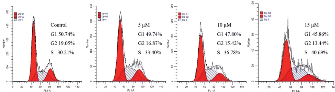
Fig. 4 Effects of compound 3b on cell cycle of MCF-7 cells. MCF-7 cells were treated with compounds 3b (0 \mu\text{M} , 5 \mu\text{M} , 10 \mu\text{M} , 15 \mu\text{M} ) for 48 h and then measured by flow cytometry.
