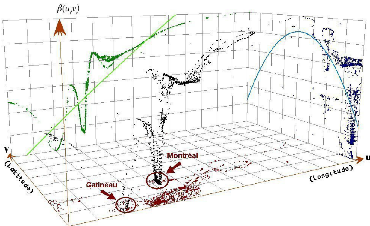
Figure 4 Trend analyses of the local relationships \beta(u, v) between ICP and the log-transformation of the length of stay (LoS).
