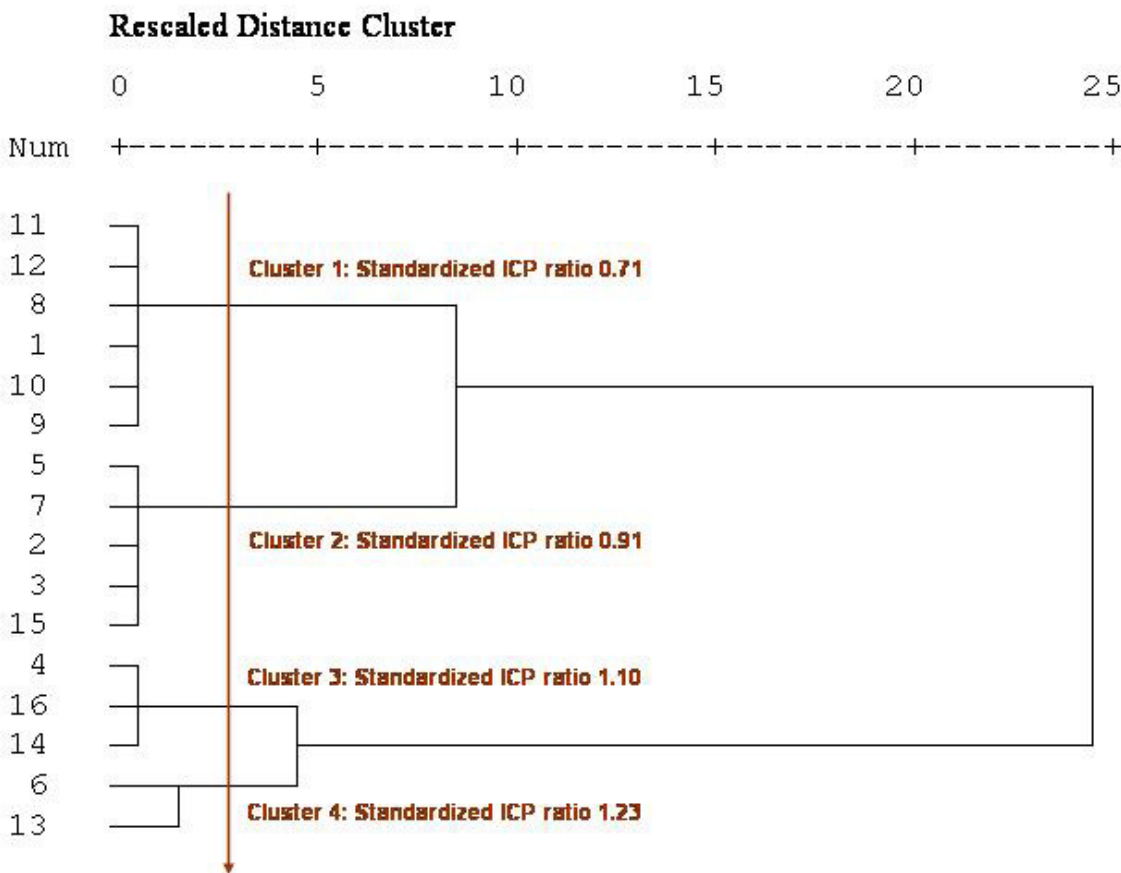
Figure 1 Dendrogram produced by a hierarchical cluster analysis of the standardized ICP ratios.
