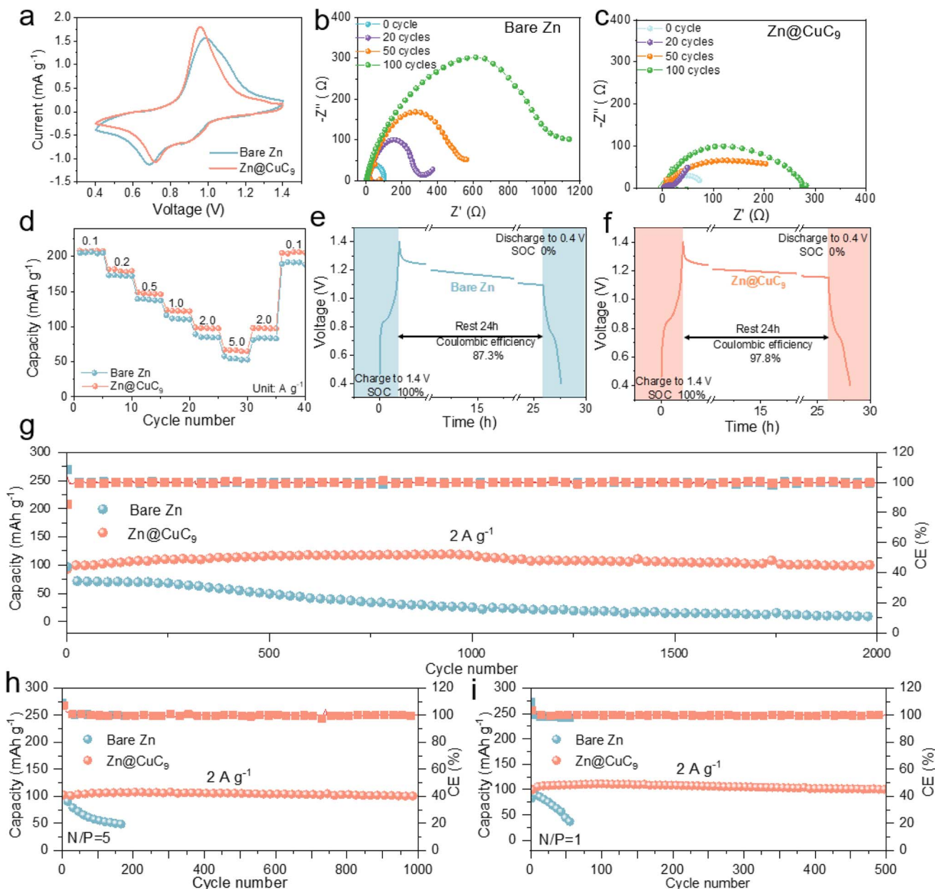
Fig. 5 (a) Cyclic voltammograms of Zn//NVO with a 1 mV s -1 scan rate. EIS plots of (b) bare Zn//NVO and (c) Zn@Cu 9 //NVO. (d) Rate performances. Self-discharge test of (e) bare Zn//NVO and (f) Zn@Cu 9 //NVO cells. (g) Cycle endurance of Zn//NVO full cells based on Zn@Cu 9 and bare Zn anodes. Cycling stability of Zn//NVO full cells at 2 A g -1 with (h) N/P ratio = 5 and (i) N/P ratio = 1.
