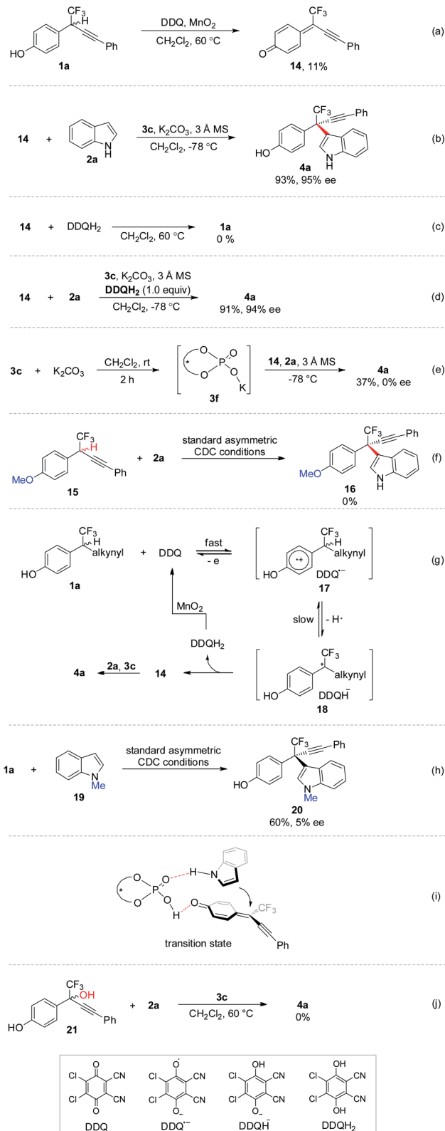
Scheme 8 Control experiments and the proposed mechanism.
