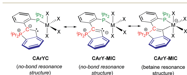
Scheme 4 Resonance structures for complexes 3–12 . The CARYC no-bond resonance structure with its C1-C2 single bond is considered less important on basis of the observed metrical parameters. The CARY-MIC notation (no-bond and betaine resonance structure) is in line with the crystallographic data and the computational results. Note that a dative C \rightarrow M bond is implied by the superimposition of both CARY-MIC resonance structures.
