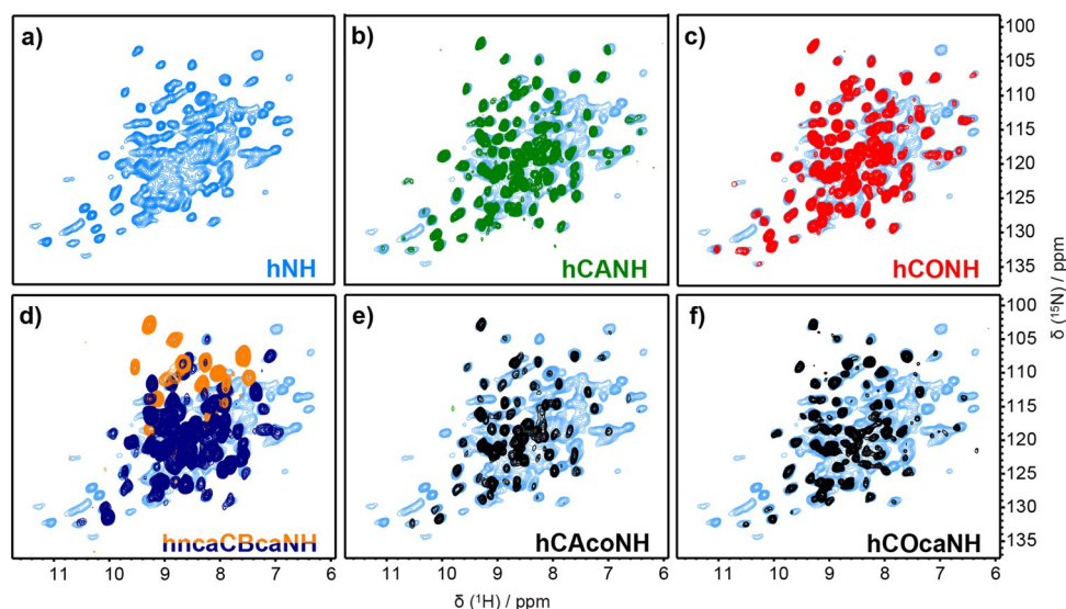
Figure 2. 2D and all planes from 3D spectra of uniformly ^2H/^{13}C/^{15}N labelled NS5A-AHD1. a) 2D hNH spectrum in light blue. b–f) Overlay of all signal-containing NH planes along the carbon dimension of hCANH, hCONH, hCAcNH, hCOcNH and hncaCBcNH 3D spectra, on the 2D hNH of panel (a) as background.
