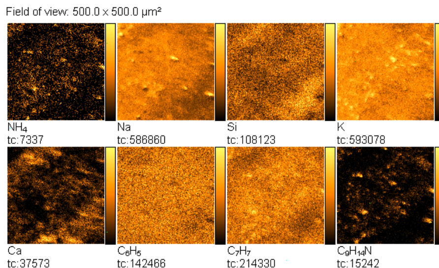
Figure 3. TOF-SIMS positive ion images ( 500 \times 500 \mu\text{m}^2 ) of fingerprint contaminated by amphetamine (deposited on glass), showing tc—total counts.
