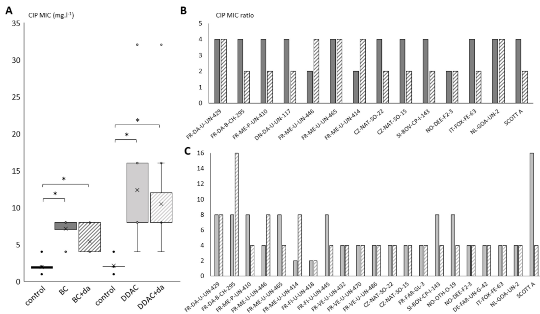
Figure 4. Stability of ciprofloxacin (CIP) MIC in Lm strains for which an increase in MIC was observed after exposition to BC (14 strains) and DDAC (21 strains). (A) Variation of CIP MIC values ( \text{mg}\cdot\text{L}^{-1} ) for Lm strains exposed to BC (dark grey) and DDAC (light grey). MIC values of corresponding strains unexposed to biocide for each biocide are also displayed (controls, black). Full bars correspond to values obtained after biocides exposition, and striped bars correspond to values obtained after an additional de-adaptation step (+da), where strains were then subcultured in growth medium without biocides to assess the stability of the MIC increase. Significant difference with control is indicated by star (*, paired T-test p -value < 0.01). Cross (x) indicates the median, circles (o) correspond to outlier values. (B) Increase MIC factor obtained for each Lm strain comparing CIP MIC after BC (B) or DDAC (C) exposure (full bars) and after de-adaptation steps (striped bars) with CIP MIC of control Lm panel.
