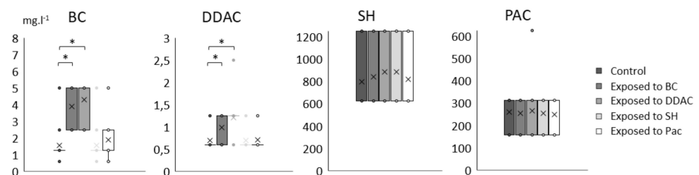
Figure 2. Variation of MIC values ( \text{mg}\cdot\text{L}^{-1} ) of benzalkonium chloride (BC), dimethylammonium chloride (DDAC), sodium hypochlorite (SH) and peracetic acid (PAC) for the 28 selected Lm strains exposed or not (control) to the 4 biocides. Significant difference with control is indicated by star (*, paired T-test, p -value < 0.01 ). Boxes range from the 25th to 75th percentile and whiskers extending below and above the box range from the lowest to the upper value, respectively. Cross ( \times ) indicates the median, circles ( \circ ) correspond to outlier values.
