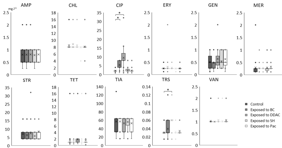
Figure 3. Variation of MIC values ( \text{mg}\cdot\text{L}^{-1} ) of the 11 antibiotics for the 28 selected Lm strains exposed or not (control) to the 4 biocides. Significant difference with control is indicated by star (*, paired T-test p -value < 0.01). Cross (x) indicates the median, circles (o) correspond to outlier values.
