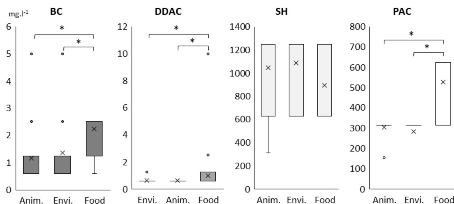
Figure 1. Distribution of minimal inhibitory concentration (MIC) values ( \text{mg}\cdot\text{L}^{-1} ) of the four biocides obtained for the 205 Lm strains depending on their ecological niches. Boxes range from the 25th to 75th percentile and whiskers extend below and above the box range from the lowest to the upper value, respectively. Cross indicates the median. Significant difference between distributions is indicated by star (Fisher’s exact test; * p -value < 0.00001). Cross (×) indicates the median, circles (○) correspond to outlier values.
