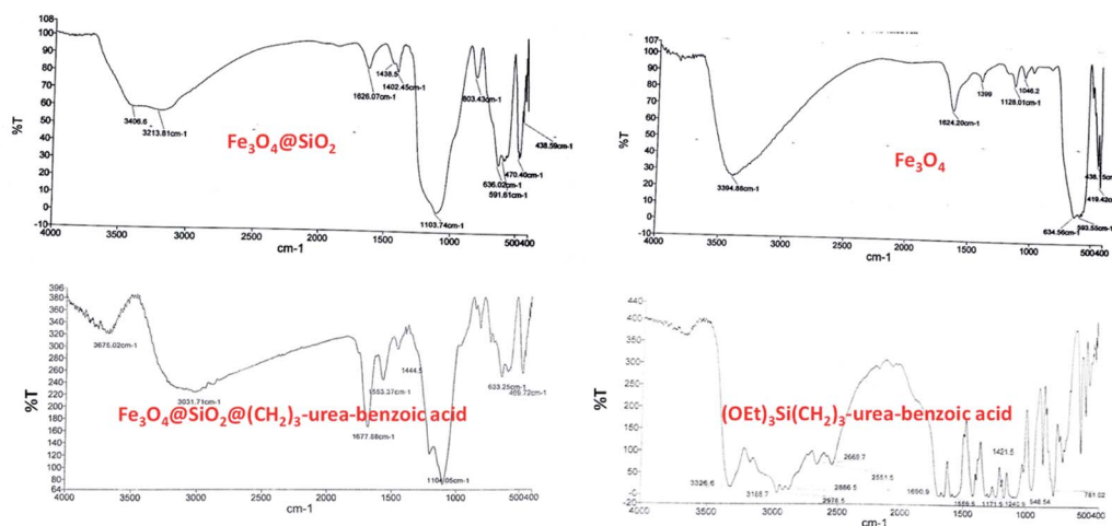
Fig. 1 FT-IR spectra of Fe 3 O 4 @SiO 2 @(CH 2 ) 3 -urea-benzoic acid and its related intermediates.
