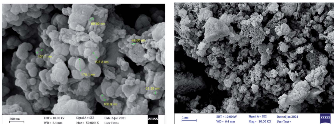
Fig. 2 SEM image of Fe 3 O 4 @SiO 2 @(CH 2 ) 3 -urea-benzoic acid.
