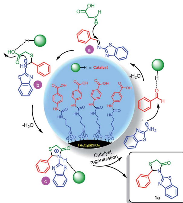
Scheme 4 The suggested mechanism for the synthesis of 1a in the presence of \text{Fe}_3\text{O}_4@(\text{CH}_2)_3\text{-urea-benzoic acid} as catalyst.
