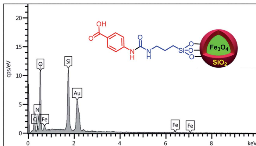
Fig. 3 EDX analysis of Fe 3 O 4 @SiO 2 @(CH 2 ) 3 -urea-benzoic acid.
