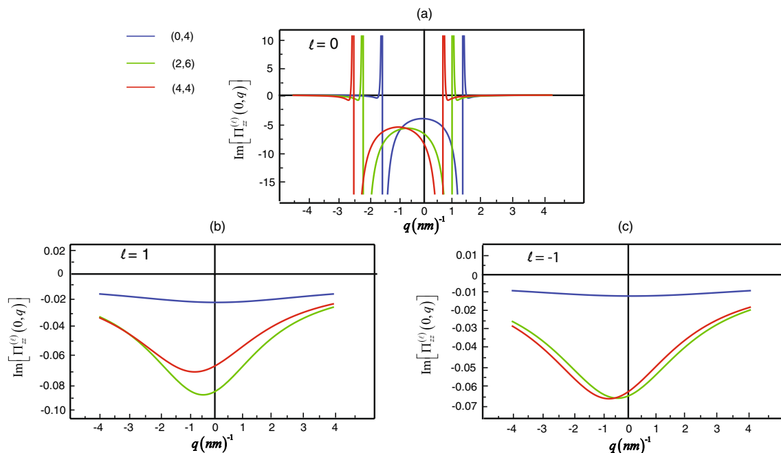
Figure 4. The simulation plots for the imaginary part of the current–current correlations \text{Im}[\Gamma_{zz}^{(\ell)}(0, q; T)] relating to the wave number q in the zigzag (0,4) (blue lines), the chiral (2,6) (green lines), and the armchair (4,4) (red lines) with different orbital number where (a) \ell = 0 , (b) for \ell = 1 and (c) for \ell = -1 .
