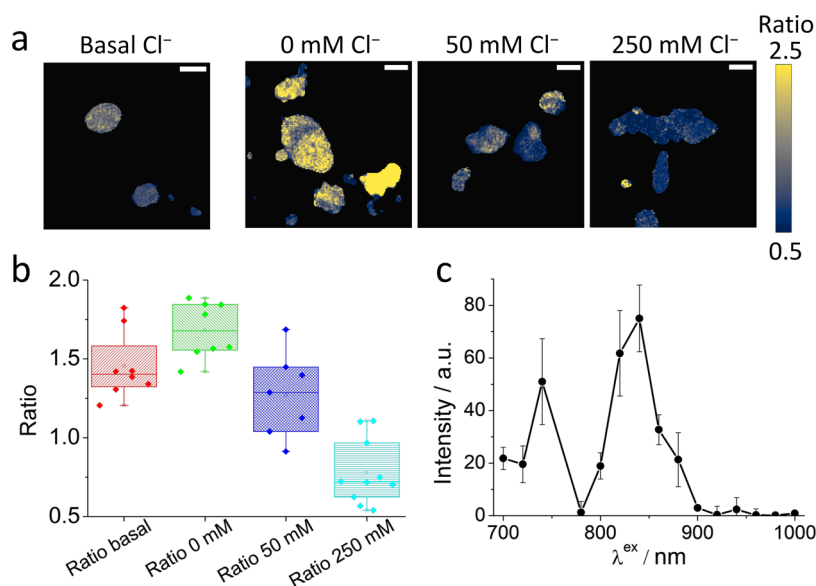
Figure 5. Two-photon excitation imaging measurements. (a) Red/green ratio maps of HEK-293 cells obtained using two-photon excitation ( \lambda_{\text{ex}} = 750 nm). The figure shows images reflecting the basal chloride concentration (left) and images of cells clamped at different chloride concentrations; scale bars: 20 \mu\text{m} . (b) The Box and whisker plot representing the average red/green ratio from the two-photon excitation data. Boxes correspond to 25 and 75%, with the horizontal bar indicating the average value. Whiskers represent the minimum and maximum values. (c) Two-photon excitation spectra measured in HEK-293 cells transfected with mBeRFP S94V-R205Y. Emission collected at 600–650 nm, and excitation ranging from 700 to 1000 nm, measured every 20 nm. The intensities were calculated by normalization to the power of the excitation source measured on the excitation pathway. Bars represent the standard error from three replicates.
