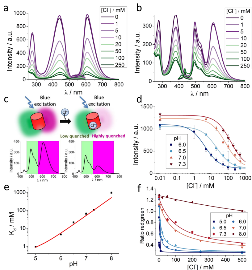
Figure 3. Influence of chloride on the spectral properties of mBeRFP and its derivatives. (a) Excitation ( \lambda emission: 610 nm) and emission fluorescence spectra of mBeRFP S94V-R205Y with an excitation wavelength of 440 nm at different chloride concentrations and pH = 6.0. (b) Excitation ( \lambda emission: 495 nm) and emission fluorescence spectra of mBeRFP S94V-R205Y with an excitation wavelength of 380 nm at different chloride concentrations and pH = 6.0. (c) Proposed scheme of the methodology of mBeRFP S94V-R205Y as a chloride biosensor. (d) Fluorescence intensity vs chloride concentration at four different pH values. Error bars represent the standard error obtained from three measurements. (e) Dependence of the dissociation constant on pH. The solid line was obtained by global data fitting to eq 3 with the following fit parameters: pK_a = 6.08 \pm 0.30 , and K_d^1 = 0.98 \pm 0.17 mM. Error bars represent the standard error. (f) Dependence of the red/green fluorescence ratio on the chloride concentration at different pH values. Error bars represent the standard error obtained from three measurements.
