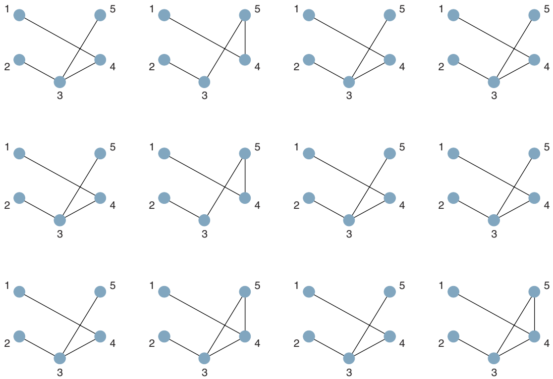
Figure 2. Graphical images of the models derived by a log-linear modelling of data from single nucleotide polymorphism (SNP)1–SNP5. A p -value threshold of 0.05 was used. The 12 graphs depict models derived from 12 bootstrap samples. A node represents a SNP and an edge denotes a pairwise interaction.
