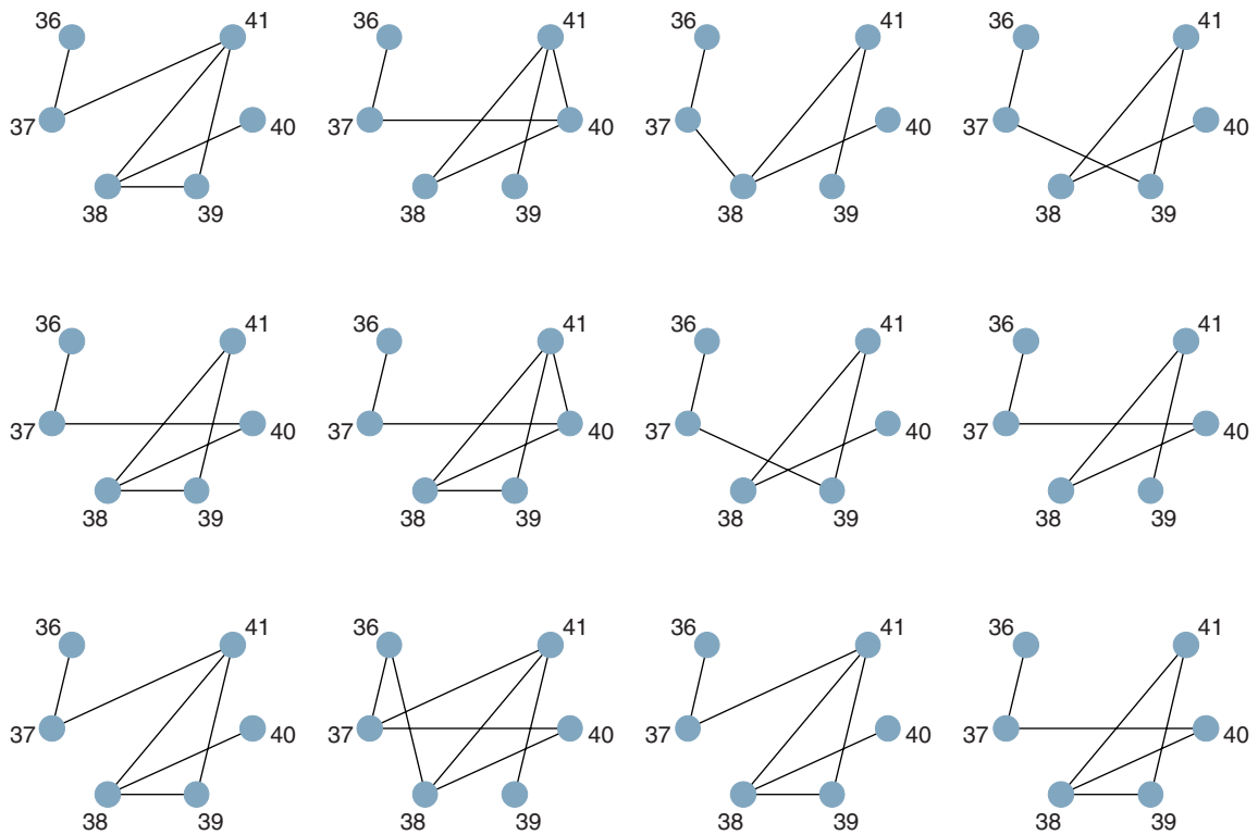
Figure 3. Graphical images of the models derived by a log-linear modelling of data from single nucleotide polymorphism (SNP)36–SNP41. A p -value threshold of 0.05 was used. The 12 graphs depict models derived from 12 bootstrap samples. A node represents a SNP and an edge denotes a pairwise interaction.
