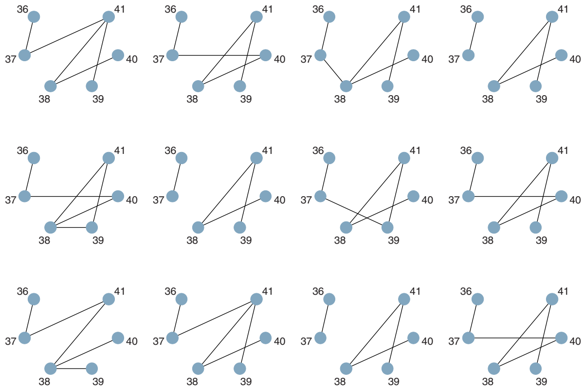
Figure 4. Graphical images of the models derived by a log-linear modelling of data from single nucleotide polymorphism (SNP)36–SNP41. A p -value threshold of 0.01 was used. The 12 graphs depict models derived from 12 bootstrap samples. A node represents a SNP and an edge denotes a pairwise interaction.
