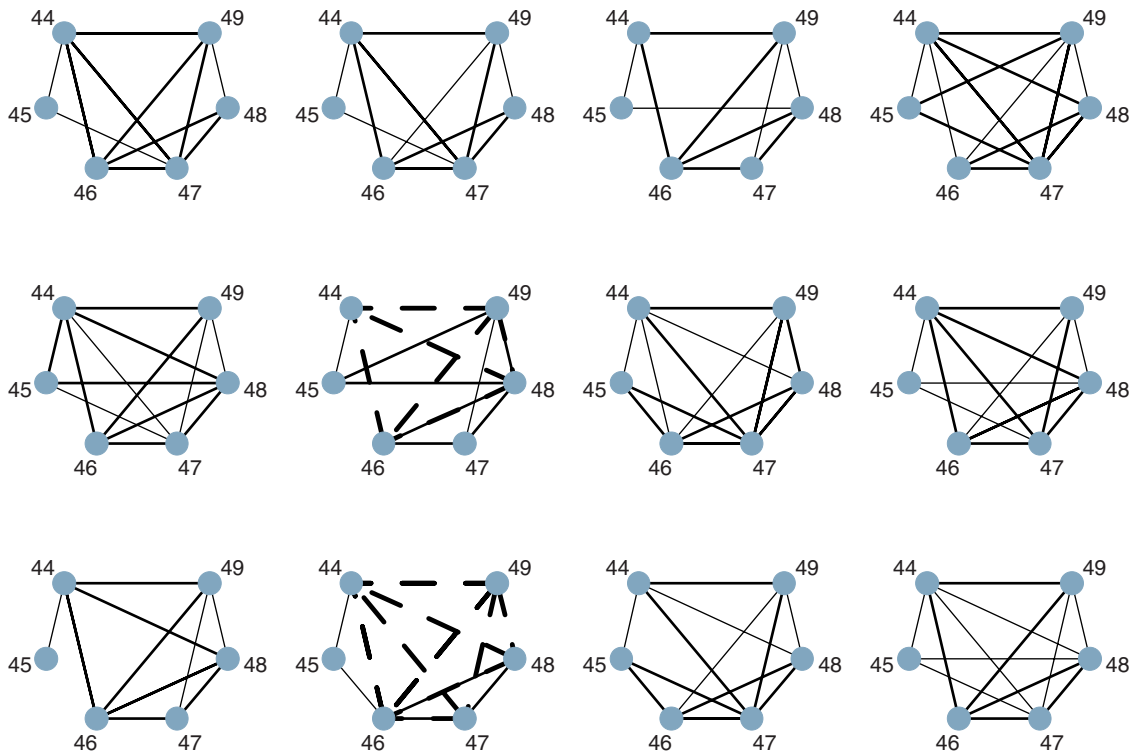
Figure 5. Graphical images of the models derived by a log-linear modelling of data from single nucleotide polymorphism (SNP)44–SNP49. A p -value threshold of 0.05 was used. The 12 graphs depict models derived from 12 bootstrap samples. A node represents a SNP and an edge denotes an interaction. Plain solid edges represent pairwise interactions; bold solid edges represent three-way interactions; broken edges in bold represent four-way interactions.
