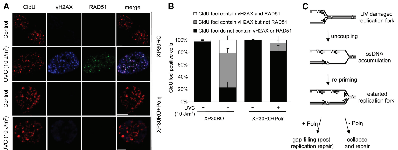
Figure 4. RAD51 co-localizes with replication sites of after UV exposure of Pol \eta^{\text{mut}} cells. (A) Representative images of UV-induced \gamma H2AX and RAD51 foci at replication forks in Pol \eta^{\text{mut}} XP30RO and restored cells pulse labelled (10 min) with CldU directly before UV exposure (10 J/m 2 ), and allowed to repair for 6 h before fixation. \gamma H2AX was used to visualize DSBs and RAD51 as an indicator of homologous recombination. Bar is 5 \mu m. (B) Quantification of co-localization of \gamma H2AX and RAD51 with CldU foci, in cells fixed 6 h after UV exposure (10 J/m 2 ). Only cells with distinct CldU foci were checked for co-localization, to only study cells replicating when irradiated. Mean and s.e.m. of four independent experiments are shown. (C) Model for the continuation of DNA replication on damaged DNA. When the replication fork runs into a UV-induced DNA lesion, the PCNA molecule is left and can be ubiquitinated to allow bypass with Pol \eta . Replication is resumed on the 5' side of the lesion, leaving a gap. In the absence of Pol \eta , the gaps are not bypassed, but collapsed into DSBs that are repaired with a pathway involving RAD51.
