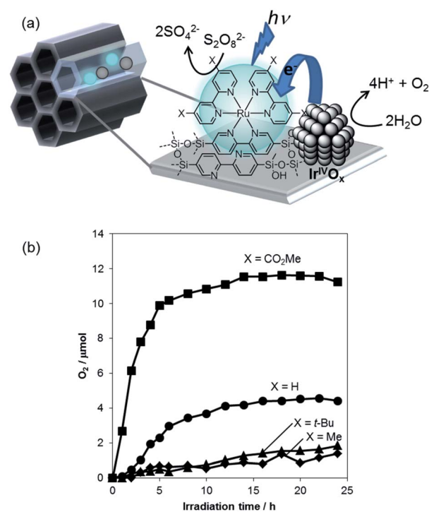
Fig. 3 (a) A schematic diagram showing the photocatalytic \text{H}_2\text{O} oxidation process. (b) Data from photocatalytic evaluations during oxygen evolution using Ru(X)-BPy-PMO ( \text{X} = \text{H}, \text{Me}, t\text{-Bu} and \text{CO}_2\text{Me} ).
