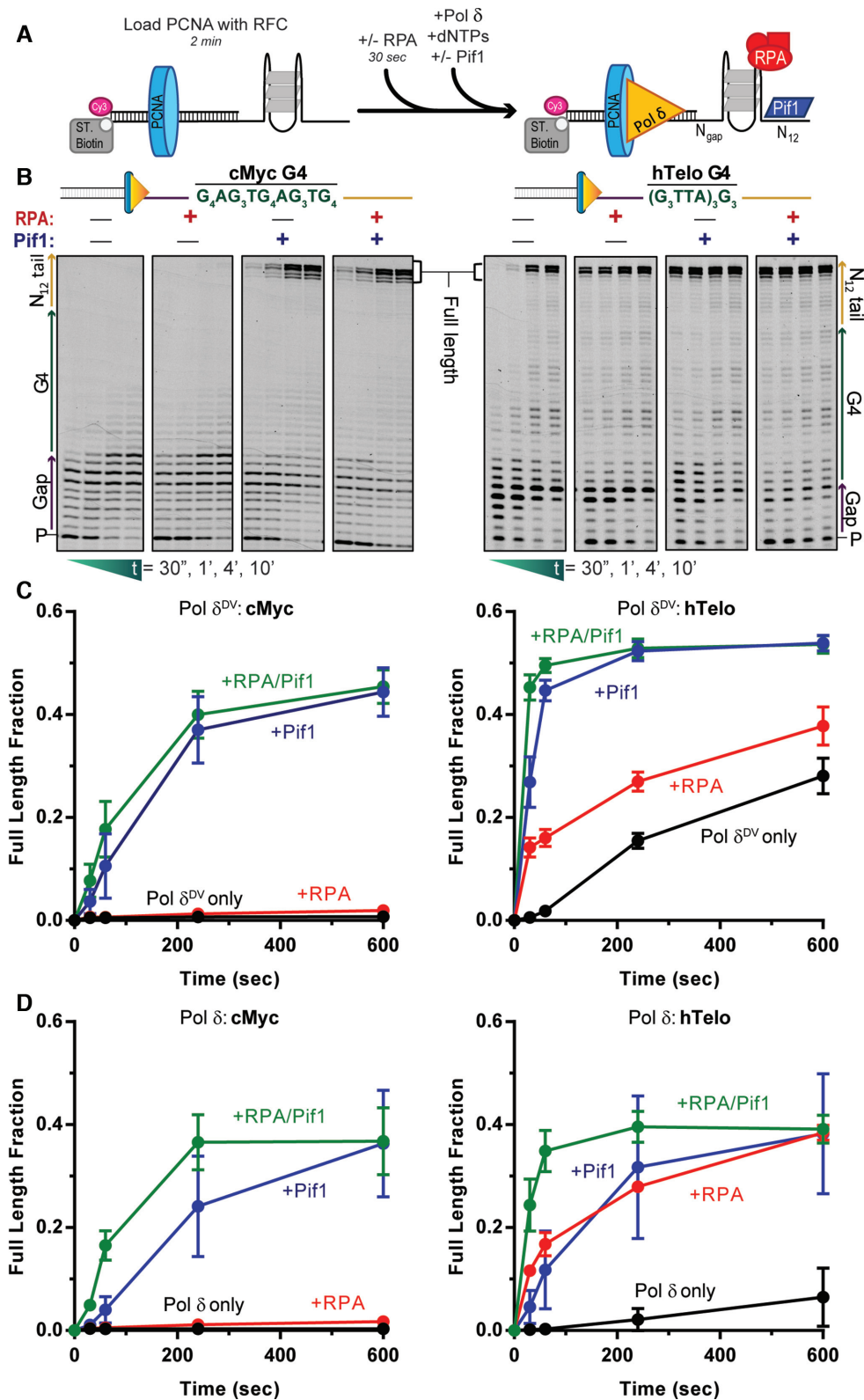
Figure 1. Pif1, but not RPA, aids Pol \delta in DNA synthesis through hTelo and cMyc G-quadruplexes. (A) Schematic of the primer extension reaction scheme. (B) Representative primer extension assay results for Pol \delta^{DV} alone (black) and in the presence of either RPA (red) or Pif1 (blue) or both (green), with cMyc (left) or hTelo (right) in the template strand. Quantifications of the fraction of full-length product generated as a function of time are shown in (C) for Pol \delta^{DV} and (D) for Pol \delta .
