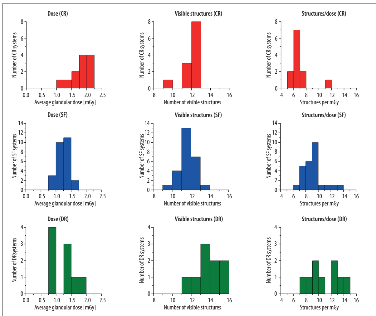
Figure 3. Average glandular dose, number of visible structures in the image of the ACR phantom, and the ratio between the number of visible structures and the average glandular dose for three groups of mammography systems.
