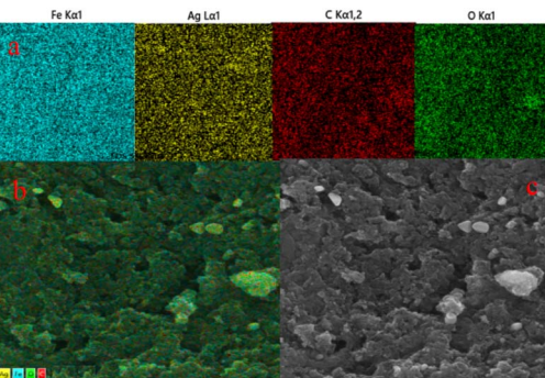
Fig. 3 (a) Color mapping of individual elements; (b) mapping and (c) SEM image of the same part of \text{Fe}_3\text{O}_4/\text{GO}/\text{Ag} .
